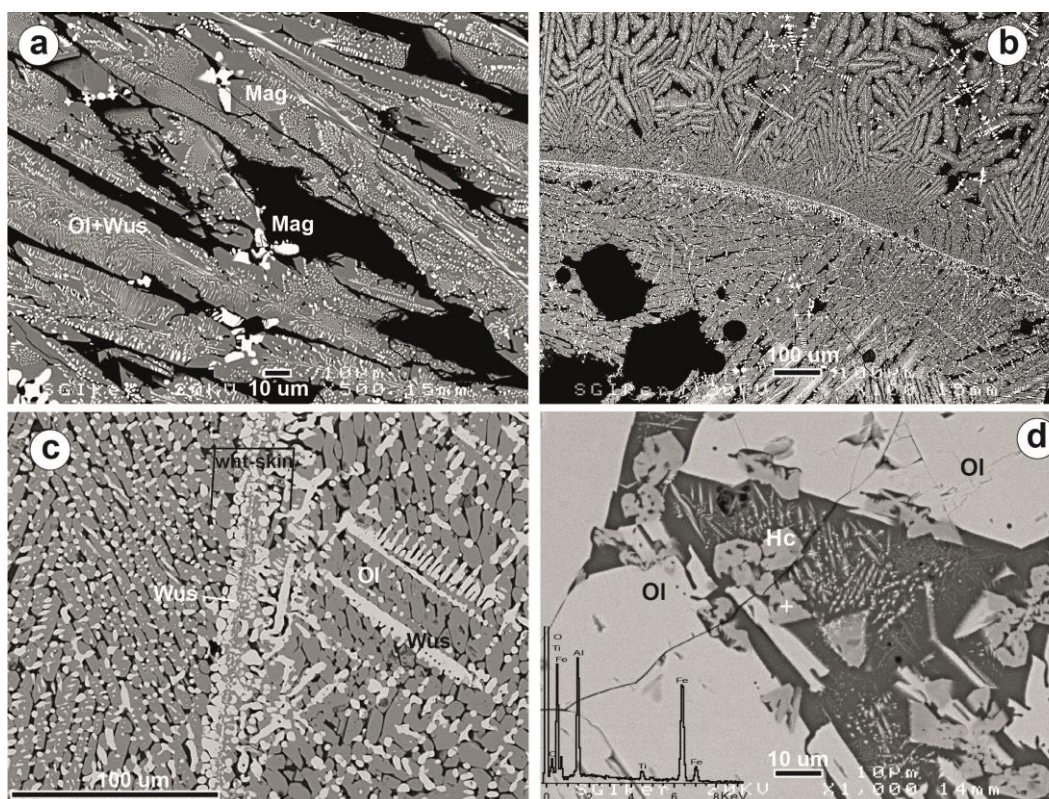
Figure 4. SEM-BSE images. (a) skeletal olivines (light-grey colors), dendritic wuestite and cruciform magnetite (white colors) in Group 1. (b) white skins and the spinifex olivines in Group 3. (c) detail of white skins. (d) polyhedral olivines (light-grey colors) and euhedral-cruciform hercynite (grey colors) and EDS spectra of hercynite taken at + spot on the image in Group 3. Abbreviations after [36]: Ol: Olivine, Wus: Wuestite, Mag: Magnetite, Wht-skin: white skin, Hc: Hercynite.
