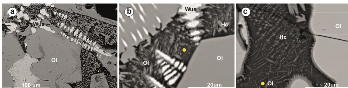
Figure 6. SEM-BSE images showing microcrystals in the vitreous matrix (a) Representative image of glass in Medieval Group 1. (b) Representative image of glass in Roman Group 4. (c) Representative image of glass in Medieval Group 3. Yellow circles correspond to 1 \mu\text{m} representative of minimum EDS analytical spot. Abbreviations after [36]: Ol: Olivine, Wus: Wuestite, Hc: Hercynite.
