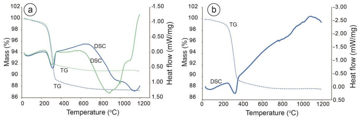
Figure 8. Thermogravimetric profiles of iron ore. (a) DSC/TG curves in environmental atmosphere of iron ore (in blue) and iron ore with quartz flux (in green). (b) DSC/TG curves in inert atmosphere.
