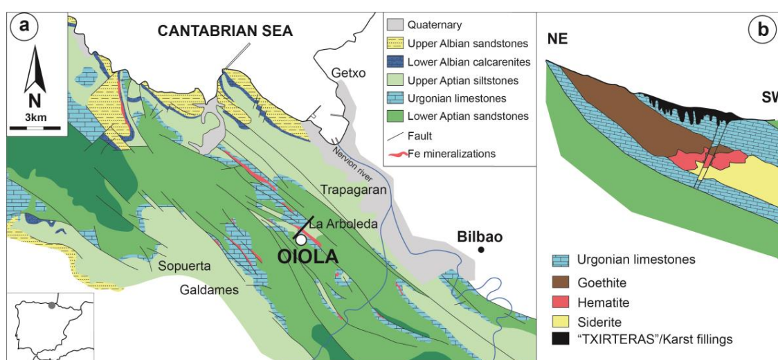
Figure 1. (a) Geographical location and geological setting of Oiola archaeological site; (b) scheme of the type of mineralization the iron oxyhydroxides (modified from [23]).
