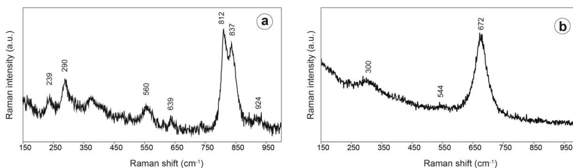
Figure 5. Raman spectra (a) Olivine spectrum. (b) White skins spectrum.
