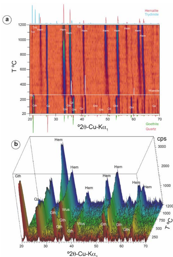
Figure 7. Thermodiffraction patterns for iron ore from Oiola heated between 30–1205 °C and from 20 to 70 °2θ range as stacked patterns showing phase transition at different temperatures. (a) stacking of 1D diffractograms; (b) stacking of 3D diffractograms. Abbreviations after [36]: Hem: Hematite, Qz: Quartz, Trd: Tydimite, Gth-Goethite: Wus: Wuestite.
