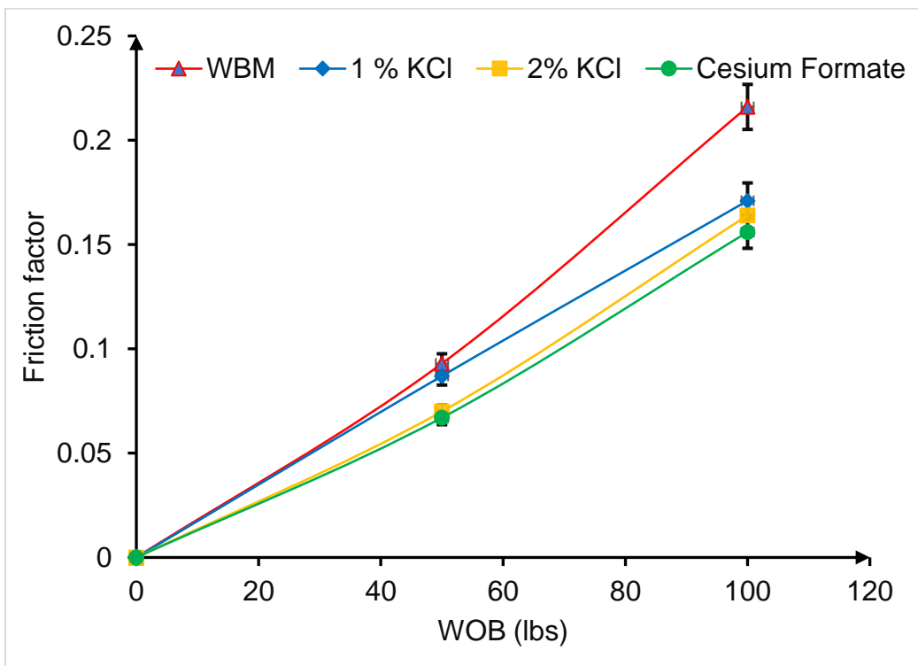
Figure 30- Effect of the tested drilling fluid systems on friction factor during drilling
