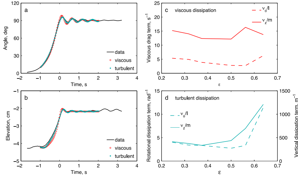
Figure 10. Results from fitting a hydrostatic iceberg capsize model to experimental data. (a) Iceberg orientation from vertical and (b) elevation of the iceberg's center of mass for an iceberg with \varepsilon = 0.5 . Black curves represent experimental data, and red and green curves are the best fit solutions for laminar viscous ( n = 1 ) and turbulent ( n = 2 ) dissipation, respectively. (c) Best fit viscous drag terms for various iceberg aspect ratios. (d) Best fit turbulent drag terms for various iceberg aspect ratios.
