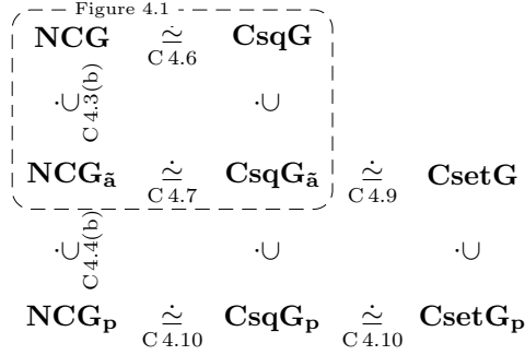
FIGURE 4.2. Some isomorphisms and strict inclusions among subcategories of \mathbf{NCG} (C=Corollary).
