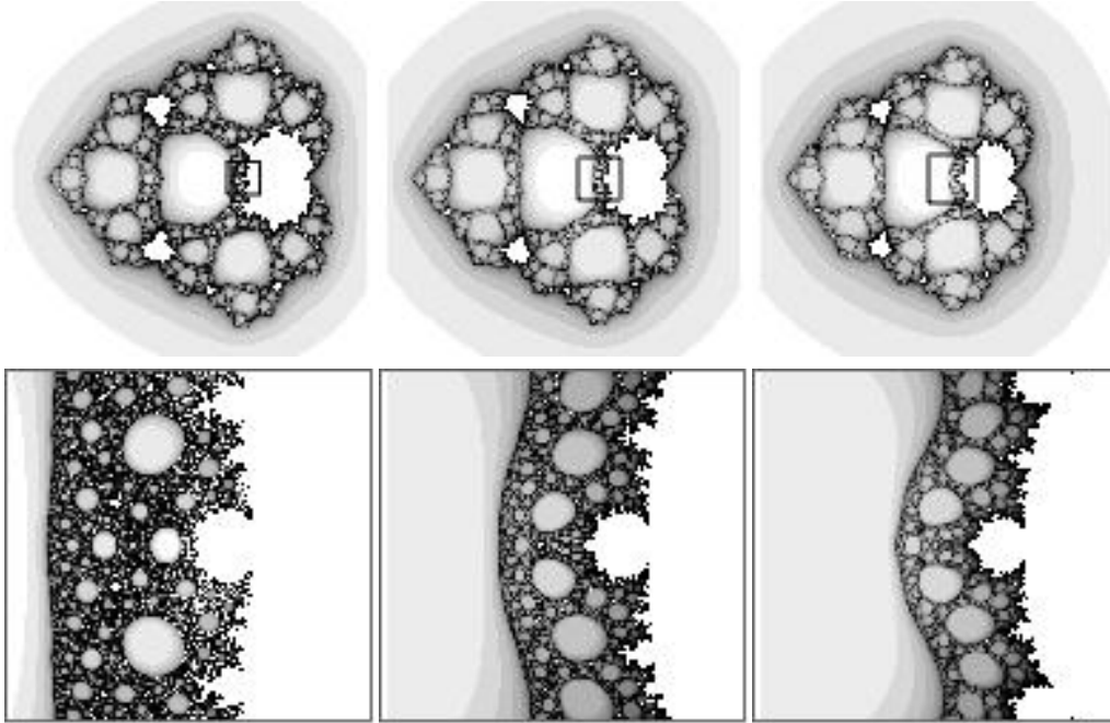
Figure 2: The top line of pictures shows the parameter planes for the family z^n + \lambda/z^d from left to right we have \langle n, d \rangle = \langle 2, 2 \rangle , \langle 2, 3 \rangle and \langle 2, 4 \rangle . The bottom line of pictures shows magnifications in the region -0.03 < \Re e \lambda < 0.03 and -0.03 < \Im m \lambda < 0.03 .
