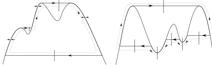
Figure 3: On the left a canard cycle with 1 breaking mechanism (jump) and exhibiting an attracting sequence. On the right a canard cycle with 3 breaking mechanisms (1 jump and 2 Hopf).
