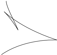
Figure 1: A planar section of the bifurcation diagram of a 3-layer canard cycle; in the bounded region 5 limit cycles are found.
