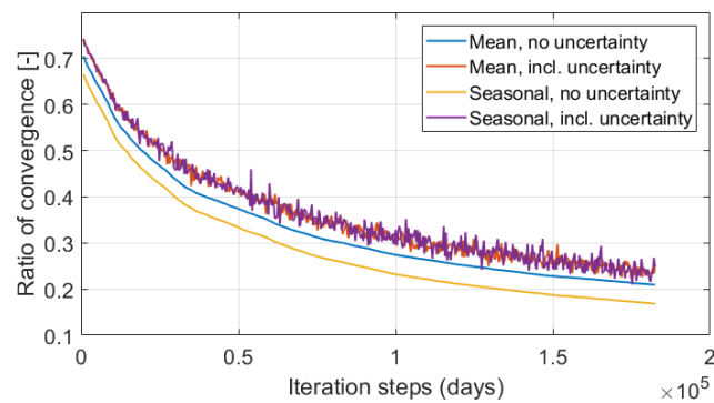
Figure B2. Convergence test in the Matura catchment, Southland, New Zealand, with inclusion of uncertainty and a Gaussian distribution over the year to include seasonality of recharge.
