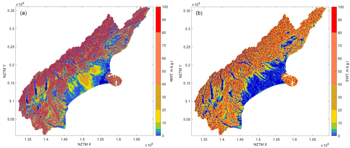
Figure 9. Water table depth of the (a) NWT and (b) EWT models in the Canterbury region.
