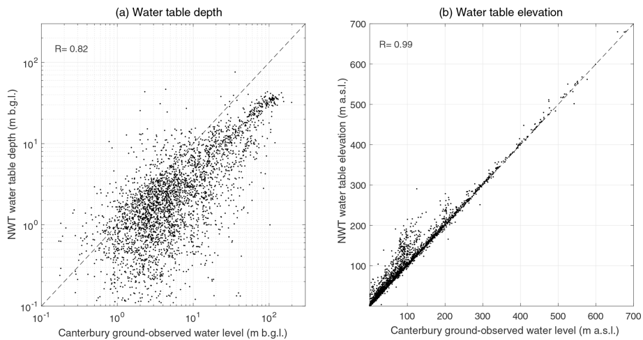
Figure 8. Correlation of NWT water table depth and water table elevation with ground observations in the Canterbury region. The dashed line is the 1 : 1 relation.
