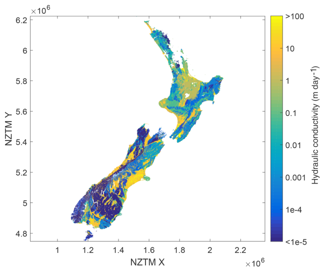
Figure 3. Hydraulic conductivity estimates for near-surface geology across New Zealand.
