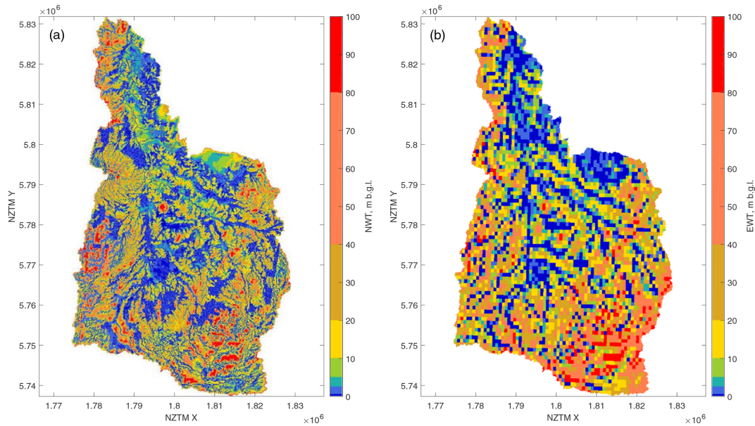
Figure 13. Water table depth of the (a) NWT and (b) EWT models in the Waipa River catchment.
