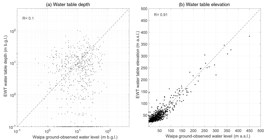
Figure 15. Correlation of EWT water table depth and water table elevation with ground observations in the Waipa River catchment. The dashed line is the 1 : 1 relation.
