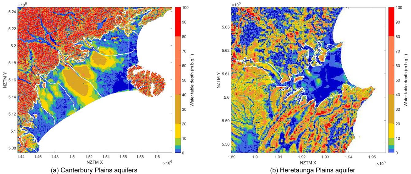
Figure 6. NWT water table depth and aquifer boundaries of White (2001) (white lines).
