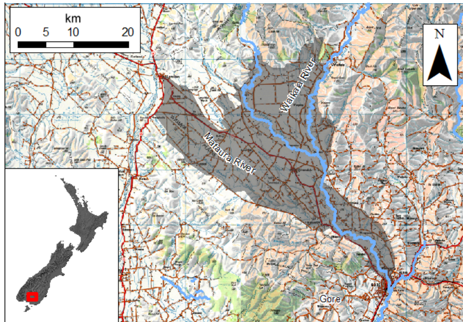
Figure B1. Model area of the Matura catchment, Southland, New Zealand.
