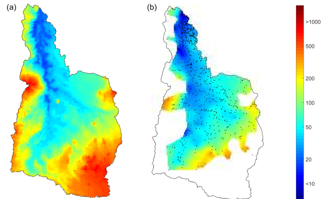
Figure 12. (a) NWT water table elevation and (b) the interpolated surface of water table elevation from ground observation in the Waipa catchment (Rawlinson, 2014). All elevations are in m a.s.l. Ground observations used for the interpolated surface are shown in black dots.
