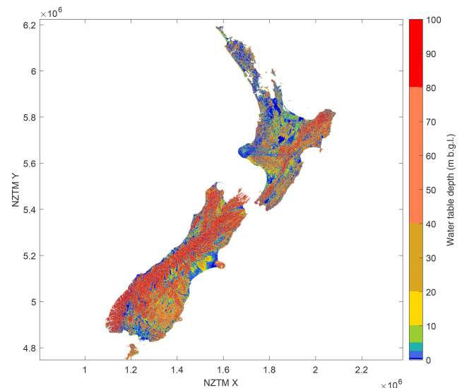
Figure 4. NWT water table depth in New Zealand.
