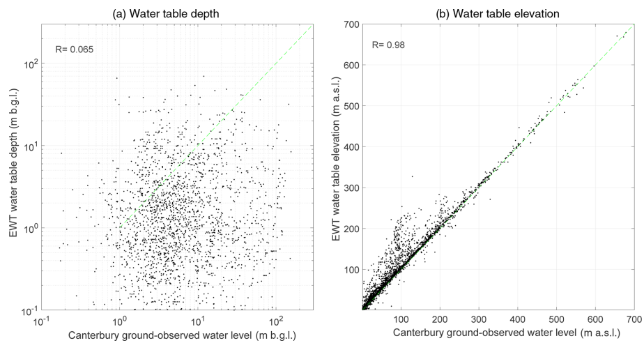
Figure 10. Correlation of EWT water table depth and water table elevation with ground observations in the Canterbury region. The dashed line is the 1 : 1 relation.
