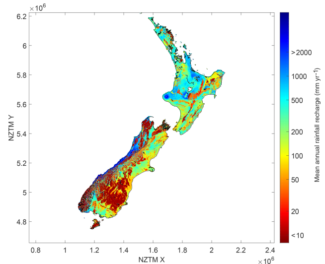
Figure 2. Mean annual rainfall recharge in New Zealand (2000–2014; Westerhoff et al., 2018).
