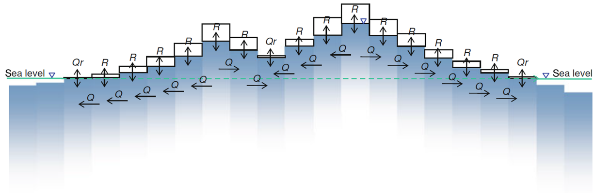
Figure A1. Schematic of the EWT model to simulate the water table at the continental scale, using recharge ( R ), horizontal groundwater flow ( Q ), groundwater discharge in rivers ( Q_r ), and sea level (boundary condition). The blue fading colours indicate the decrease of hydraulic conductivity with depth (Fan and Miguez-Macho, 2010b, their Fig. 4a).
