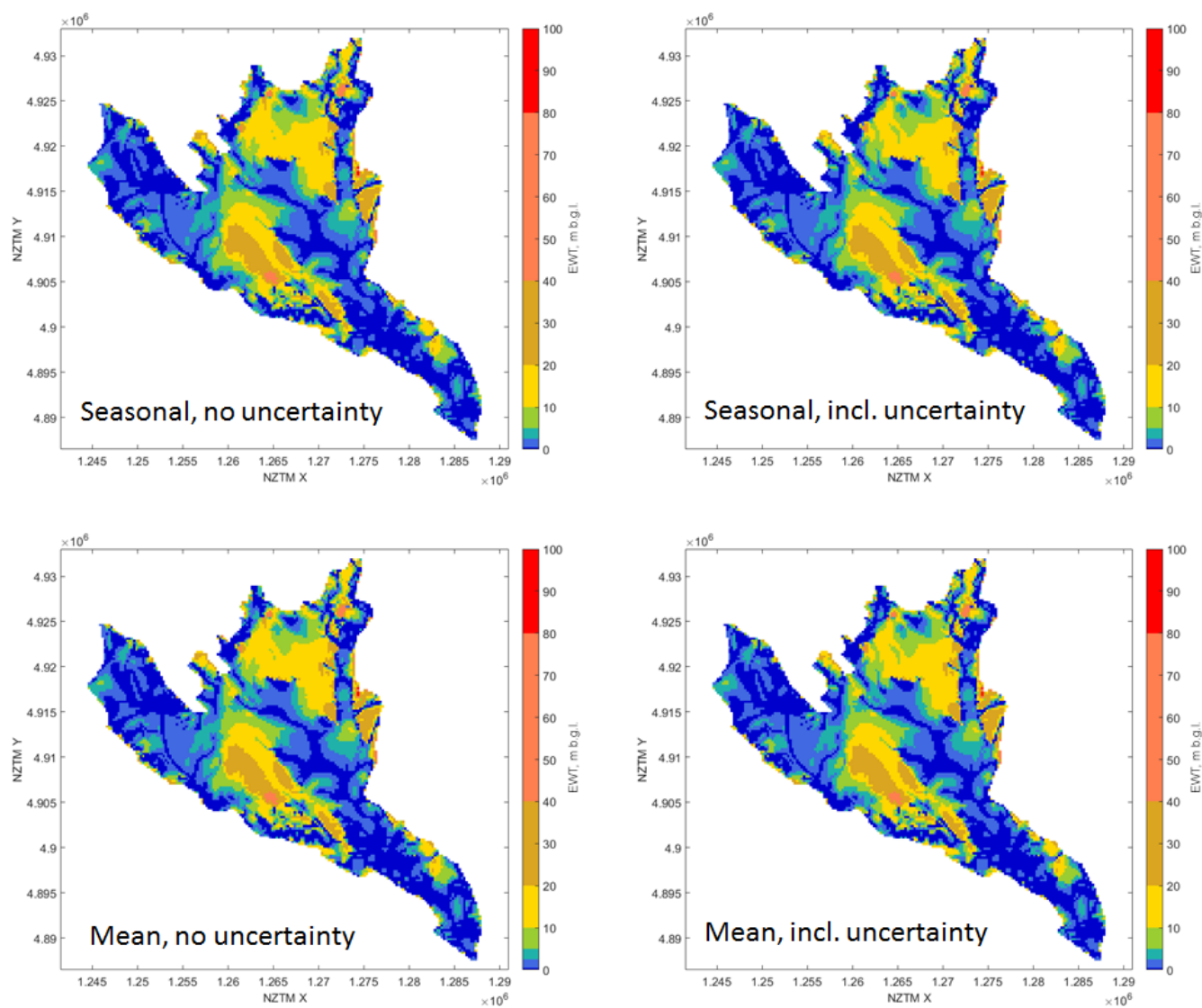
Figure B3. Convergence test in the Matura catchment, Southland, New Zealand, with inclusion of uncertainty and a Gaussian distribution over the year to include seasonality of recharge.
