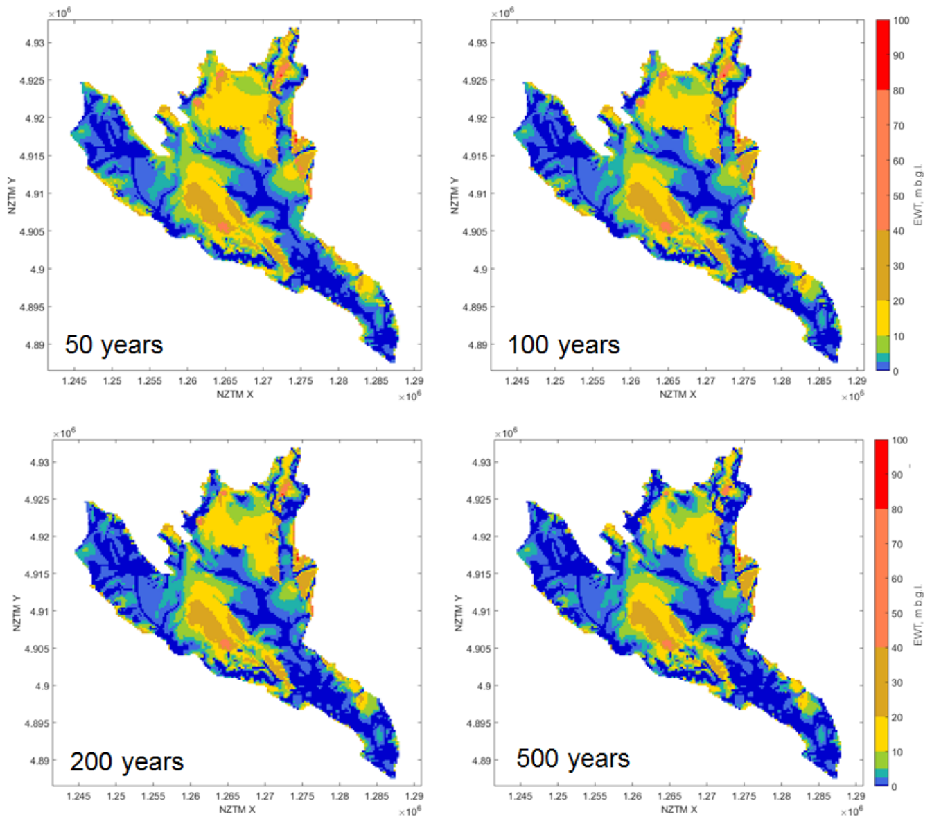
Figure B4. Convergence test in the Matura catchment, Southland, New Zealand, with model runtimes of 50, 100, 200, and 500 years.
