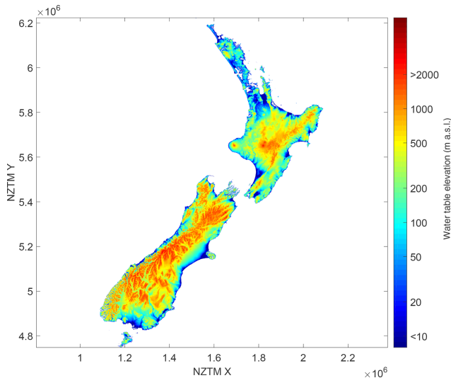
Figure 5. NWT water table elevation in New Zealand.
