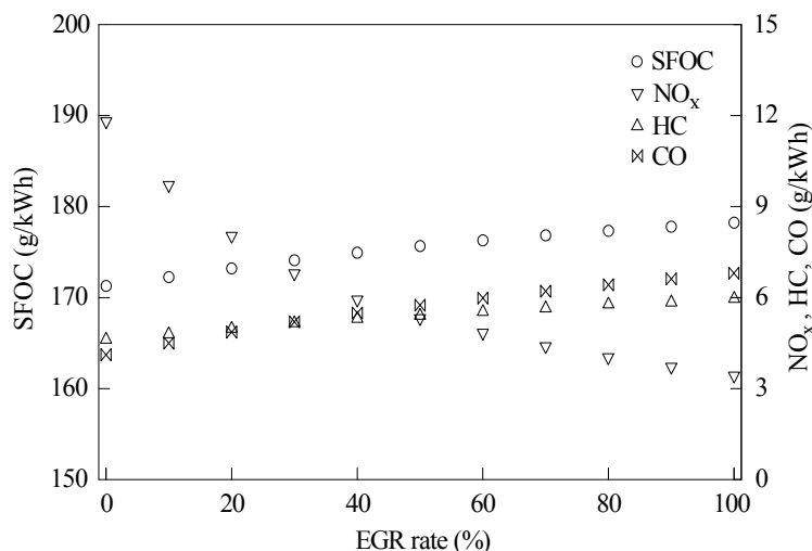
Fig. 7 SFOC, \text{NO}_x , HC and CO against the EGR rate.
