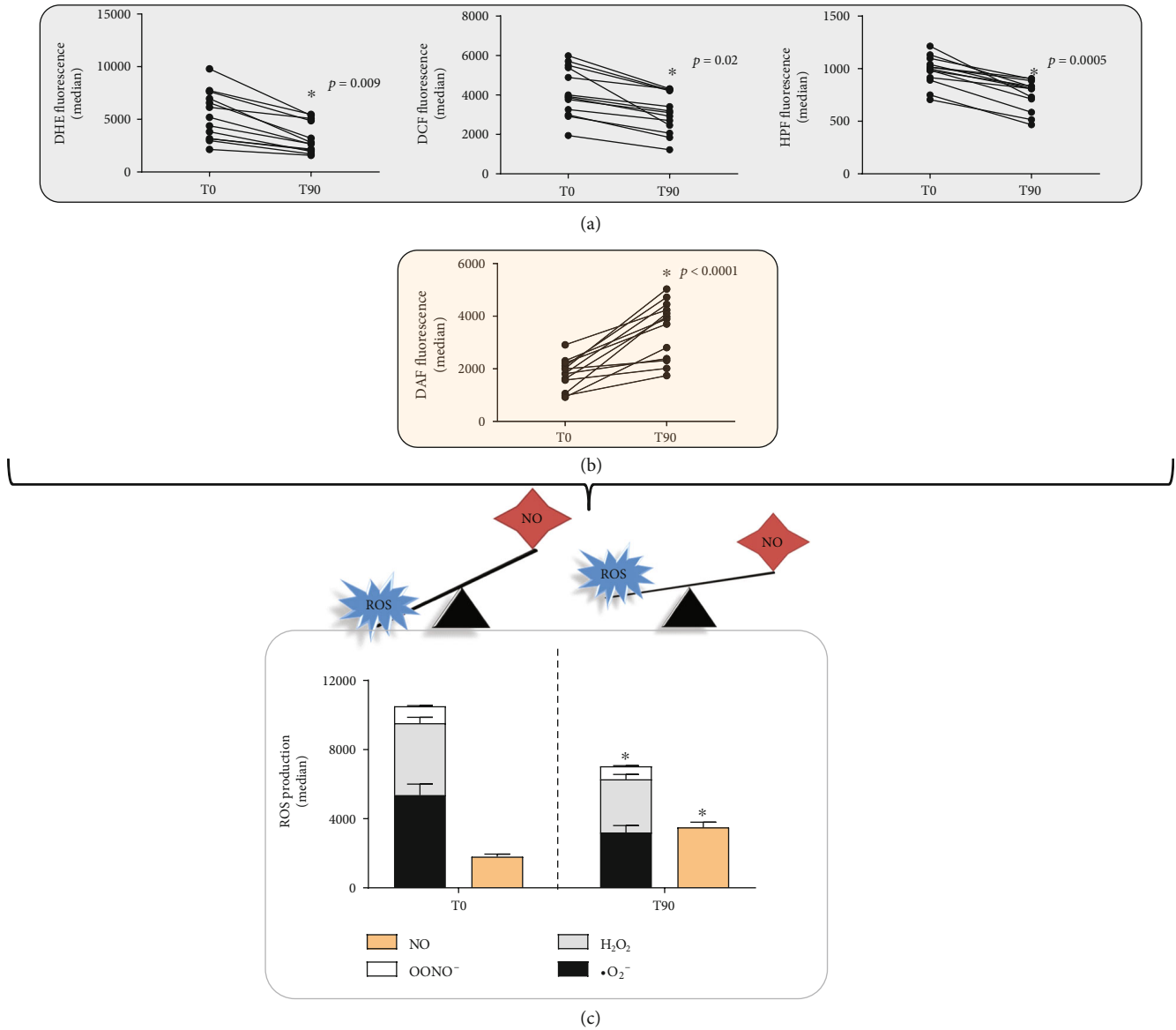
FIGURE 4: Superoxide anion, hydrogen peroxide, peroxyntirite/hydroxyl radical, and nitric oxide levels measured by specific biomarkers commonly used to evaluate ROS (DHE, DCF, HPF, and DAF staining, respectively). Records of ROS production were made before and after 90 days of the probiotic supplementation. Note a marked recovery of the ROS imbalance after the treatment. The results were expressed as mean \pm SEM ( n = 13 ). * p < 0.05 compared to T0.
