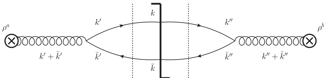
Figure 3. The cross section for producing a q\bar{q} pair as written in eq. (3.3). The vertical dotted lines denote the effective positions of the Wilson lines, which shift the quark and antiquark momenta from k, \bar{k} in the final state to k', \bar{k}' in the amplitude and k'', \bar{k}'' in the complex-conjugate amplitude. Note that the form of the amplitude (2.7) makes it possible to write all time orderings as if the q\bar{q} pair passed through the shockwave as illustrated here.
