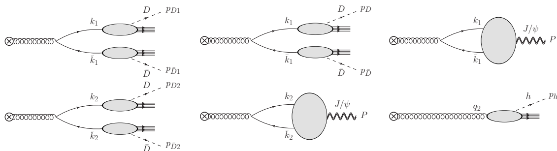
Figure 8. A few examples of how the partonic cross sections calculated in this paper can hadronize into the heavy flavor sector. The partonic (c\bar{c}) cross section could hadronize into the open heavy flavor sector such as (D\bar{D}) ( D\bar{D} ) (left panel, eq. (5.2)) or may include heavy quarkonia such as (D\bar{D}) ( J/\psi ) (center panel, eq. (5.6)). The partonic (c\bar{c}) G cross section could hadronize similarly, but include a light hadron h produced by the gluon, as in (J/\psi)h (right panel, eq. (5.7)).
