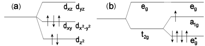
FIG. 2. Level scheme representing (a) the prismatic crystal field levels for a Co 4+ cation and (b) the electronic structure for a Co 4+ cation in a trigonally distorted OH environment. The splitting of the t_{2g} levels caused by this distortion can be observed.
