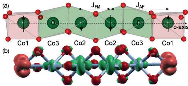
FIG. 1. (Color online) (a) Schematic picture of the structure of the CoO 3 chains in Sr 6 Co 5 O 15 obtained using VESTA (Ref. 13). OH environments for both Co2 and Co3 atoms as well as the TP one for Co1 are shown. We also show the ferromagnetic (FM) coupling ( J_{FM} ) between neighbor Co2 atoms and the antiferromagnetic (AF) one between Co2 and Co1 mediated by a nonmagnetic Co3 ( J_{AF} ). (b) Three-dimensional plot of the spin density in the FiM ground state, isosurface at 0.1 \text{ e}/\text{\AA}^3 obtained using XCrysDen (Ref. 14). Spin-up density corresponds to Co1 and spin-down density corresponds to both Co2 and Co3.
