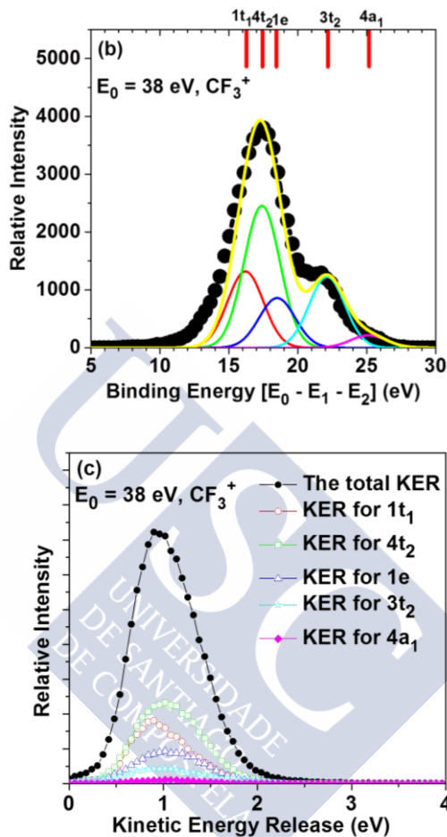
Figure 5.4(continued): (b) The binding energy spectrum. The solid circles with error bars are the experimental data. The solid red, green, blue, cyan, and magenta solid lines show the contributions of the orbitals 1t_1 , 4t_2 , 1e , 3t_2 and 4a_1 respectively. The solid yellow line shows the sum of the Gaussians. The vertical red lines on the top of the figure indicate the energies of the different molecular orbitals that contribute to form CF_3^+ ions, (c) The total KER distribution and KER for 1t_1 (BE: 13–16 eV), 4t_2 (BE: 16–18.5 eV), 1e (BE: 18.5–20.5 eV), 3t_2 (BE: 21–23 eV), and 4a_1 (BE: 24.5–27 eV) orbitals.
