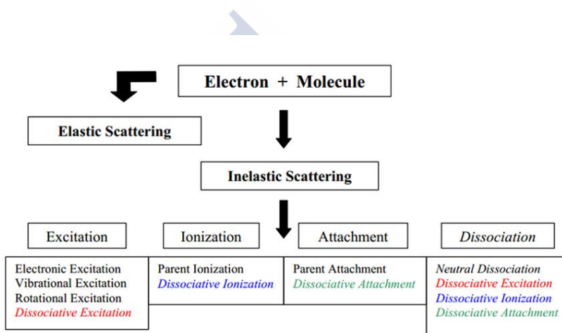
Figure 2.1: The different types of elastic and inelastic scattering processes.
