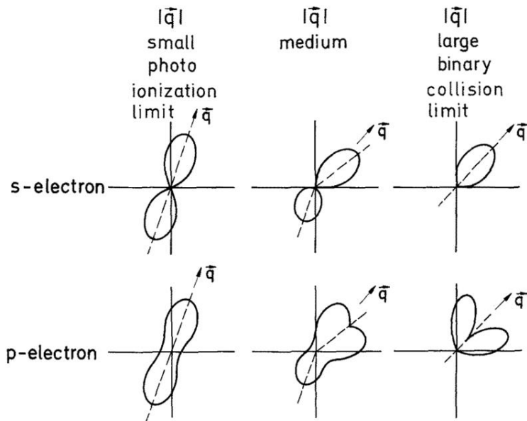
Figure 2.6: Typical triple differential cross sections for the ejection of an atomic s or a p electron for small (left), medium (middle) and large (right) momentum transfer in the range of high impact energies [18].
