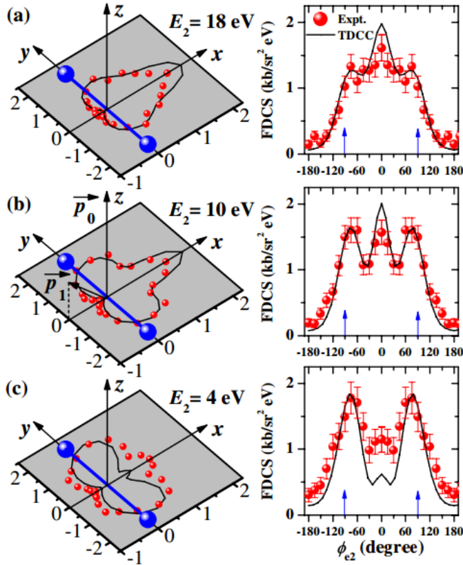
Figure 2.9: Fully differential cross sections for the ionization of aligned H_2 molecules with energy (a) E_1 = E_2 = 18 eV, (b) E_1 = 26/E_2 = 10 eV, (c) E_1 = 32/E_2 = 4 eV, and with one electron emission angle fixed to \theta_{e1} = -50^\circ [ \vec{p}_1 indicated in (b)] as a function of the emission angle of the second electron in the perpendicular ( x - y ) plane. The H_2 molecule is aligned as indicated by the (blue) spheres in the left column along the y -axis ( \theta_{Mol} = 90^\circ, \phi_{Mol} = 90^\circ ). The left column displays the FDCS in a polar plot, Cartesian plots are shown in the right column [56].
