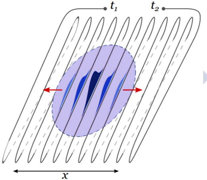
Figure 3.6.: Schematic view of a delay-line used for position sensitive detector.
