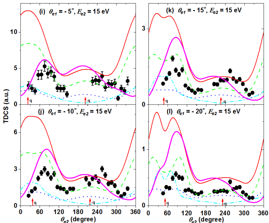
Figure 6.4(continued): (i)-(l): Scattering ( xz ) plane triple-differential cross sections (TDCS) for ionization of the 1\pi_g , 1\pi_u , and 3\sigma_u orbitals of \text{CO}_2 as a function of the ejected electron emission angle \theta_2 for scattering angles \theta_1 = -5^\circ, -10^\circ, -15^\circ, -20^\circ and for ejected-electron energies E_2 = 15 eV. Experimental data (solid circles with error bars) and theoretical results from MCDW-WM (thick magenta line), and MCDW (thin red line) are summed TDCS. Individual TDCS for 1\pi_g (green dashed line), 1\pi_u (blue dotted line), and 3\sigma_u (cyan dash dotted line) orbitals are obtained by MCDW method. The vertical arrows indicate the momentum transfer direction +q and its opposite -q .
