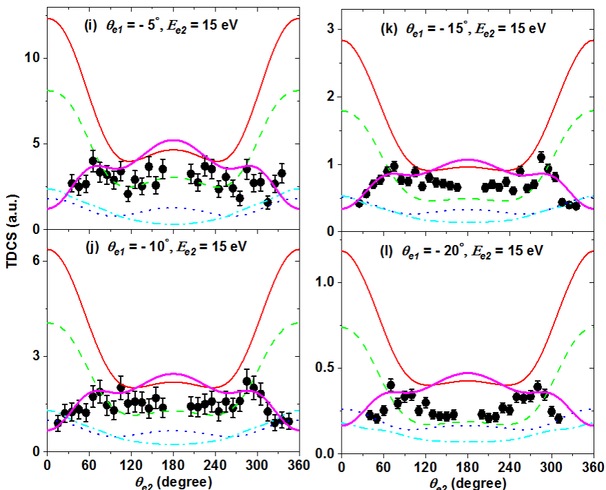
Figure 6.5(continued): (i)-(l): Perpendicular ( yz ) plane triple-differential cross sections (TDCS) for ionization of the 1\pi_g , 1\pi_u , and 3\sigma_u orbitals of \text{CO}_2 as a function of the ejected electron emission angle \theta_2 for scattering angles \theta_1 = -5^\circ, -10^\circ, -15^\circ, -20^\circ and for ejected-electron energies E_2 = 15 eV. Experimental data (solid circles with error bars) and theoretical results from MCDW-WM (thick magenta line), and MCDW (thin red line) are summed TDCS. Individual TDCS for 1\pi_g (green dashed line), 1\pi_u (blue dotted line), and 3\sigma_u (cyan dash dotted line) orbitals are obtained by MCDW method.
