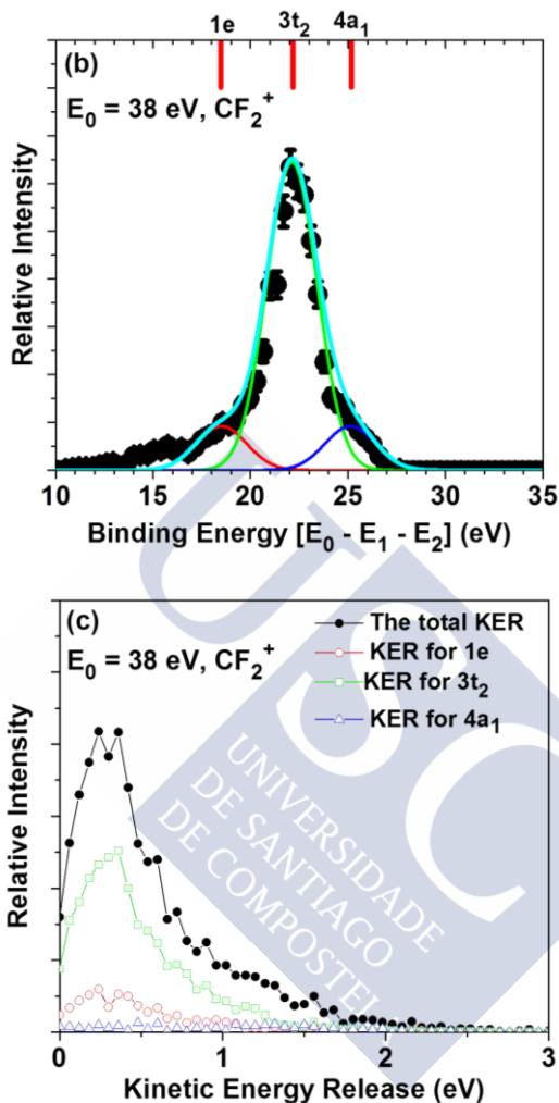
Figure 5.6 (continued): (b) The binding energy spectrum. The solid circles with error bars are the experimental data. The red, green, and blue solid lines show the contributions of the orbitals 1e , 3t_2 and 4a_1 respectively. The solid cyan line shows the sum of the Gaussians. The vertical red lines on the top of the figure indicate the energies of different molecular orbitals which contribute to the \text{CF}_2^+ ion yield, (c) The total KER distribution and KER for 1e (BE: 16–20 eV), 3t_2 (BE: 20–24 eV) and 4a_1 (BE: 25–28 eV) orbitals.
