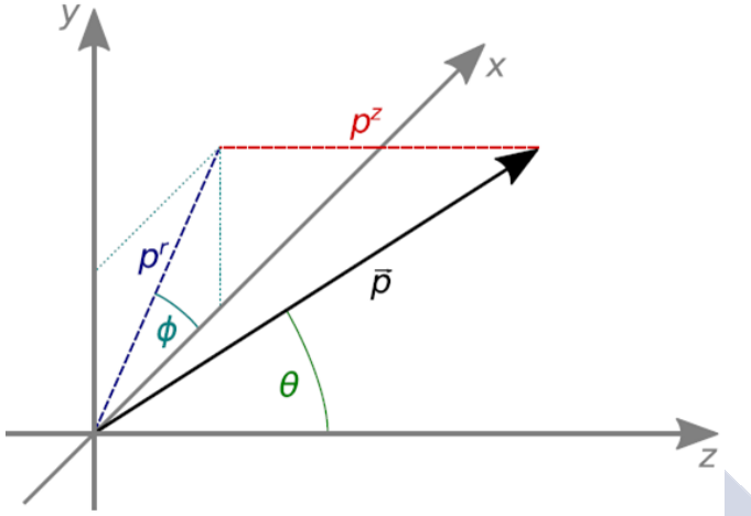
Figure 4.9: Overview of the components of a momentum vector in cylindrical coordinates.
