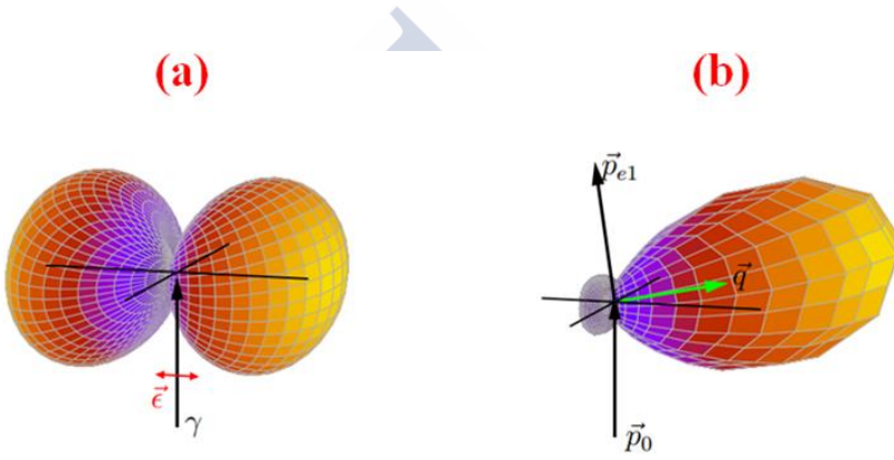
Figure 2.5.: Angular distribution of ejected electrons for: (a) photoionization and (b) electron impact ionization of helium. In (a) the propagation direction of the light field is denoted by \gamma and its polarization by \vec{\epsilon} , while in (b) the projectile electron momentum is denoted by \vec{p}_0 , the scattered projectile momentum and the momentum transfer by \vec{p}_{e1} and \vec{q} , respectively [92].
