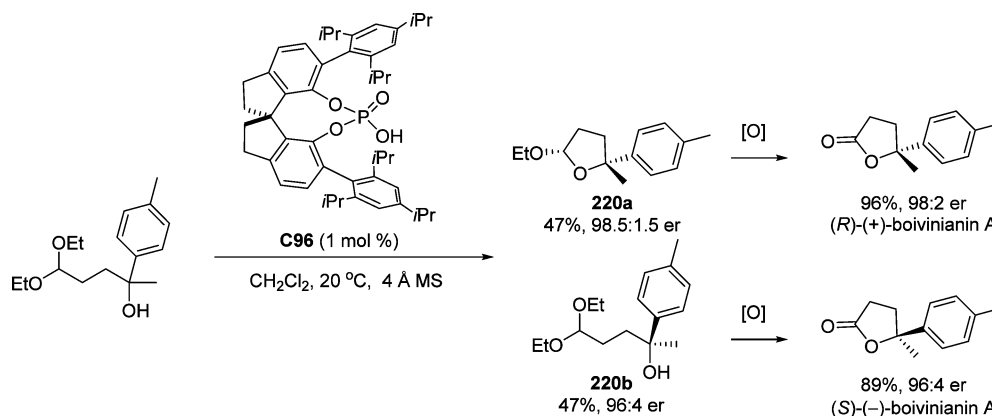
Scheme 123. Asymmetric Synthesis of trans -Fused Butyrolactones 224
