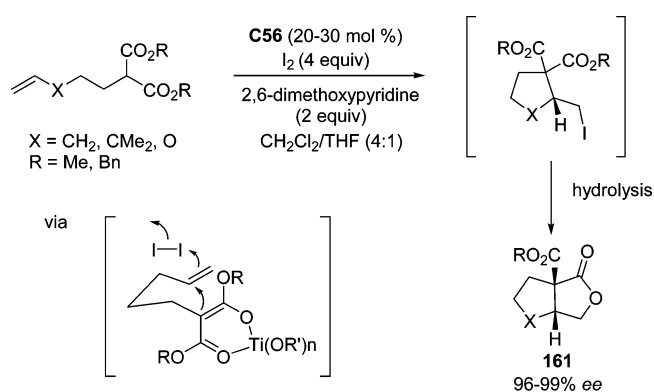
Scheme 82. Asymmetric Synthesis of Fused \gamma -Butyrolactones through Iodolactonization of Malonate with I 2
