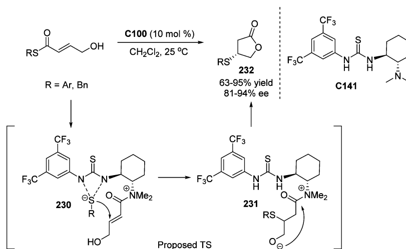
Scheme 126. Bifunctional Aminothiourea Catalyzed Asymmetric Isomerization of \omega -Hydroxy- \alpha,\beta -Unsaturated Thioesters
