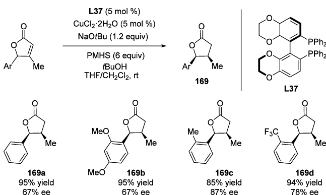
Scheme 80. Copper-Catalyzed Conjugate Reduction Synthesis of \gamma -Aryl-Containing \beta -Substituted Butenolides
