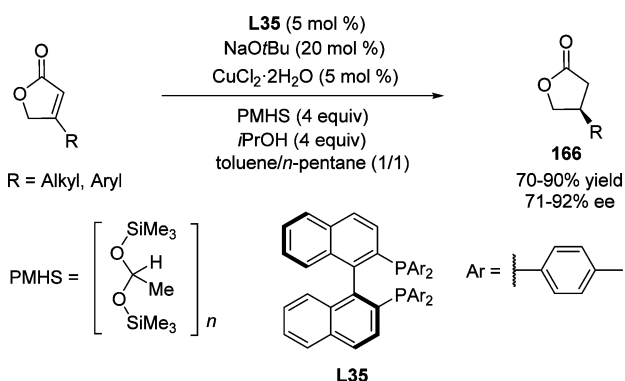
Scheme 78. Copper-Catalyzed Asymmetric 1,4-Reduction of \beta -Substituted \gamma -Butenolides
