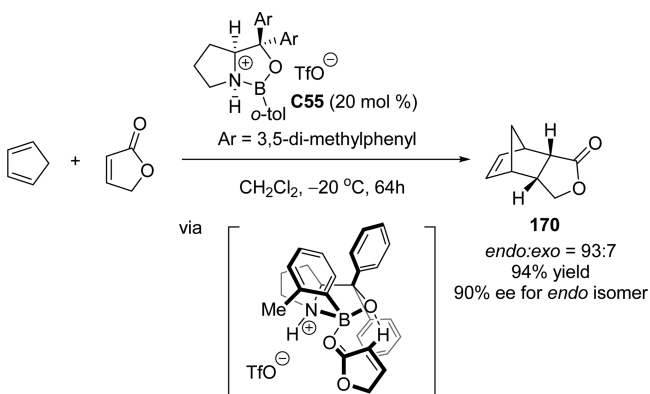
Scheme 81. Cationic Oxazaborolidine Catalyzed Asymmetric Diels–Alder Reaction of Butenolide
