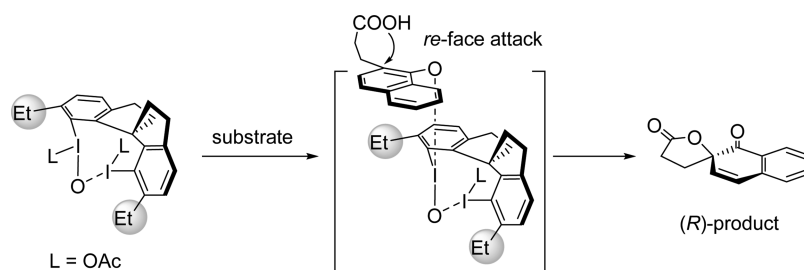
Scheme 118. Proposed Transition-State Model for the Formation of Spirolactone Products (Adapted from ref 354. Copyright 2013 American Chemical Society.)
