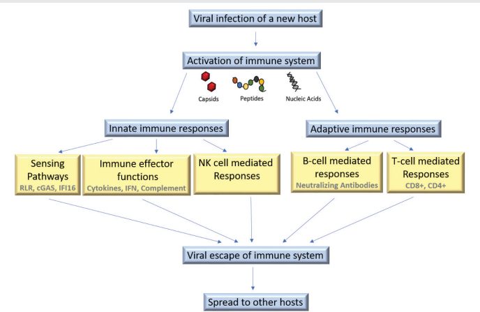
Figure 1: Schematic representation of the main responses to viral infection.
