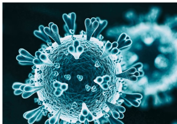
Figure 1. Morphology of the coronavirus (Source: The Scientist ) (Olona 2020)
