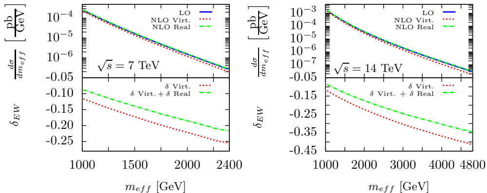
Fig. 1. – Weak corrections to Z+2 jets in the ATLAS setup of eqs. (1) at LHC energies of \sqrt{s} = 7 and 14 TeV. The upper panels show the effective mass distribution at LO (solid blue line), at NLO including only virtual one loop weak corrections (dotted red line) and at NLO including only real \mathcal{O}(\alpha) corrections (dash-dotted green line). The lower panels show the relative effects ( \delta_{EW} = \frac{d\sigma^{NLO} - d\sigma^{LO}}{d\sigma^{LO}} ) of virtual weak corrections (dotted red line) and the effect of the sum of virtual and real weak corrections (dash-dotted green line).
