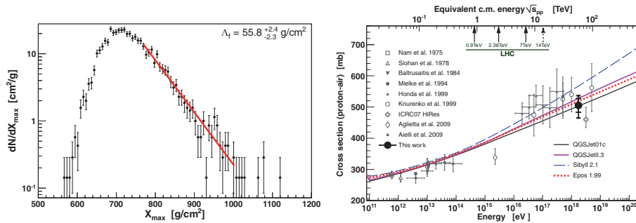
Fig. 6. – On the left, unbinned likelihood fit of \Lambda_f to the tail of the X_{\max} distribution. On the right, the resulting \sigma_{\text{p-air}} is compared to other measurements and model predictions. The inner error bars are statistical only, while the outer include all systematic uncertainties for a helium fraction of 25% and 10 mb photon contamination systematics [9, 30].
