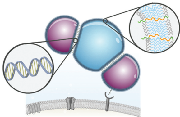
Scheme 1 Synthetic nanocompartments (polymersomes, shown in blue and magenta) assembled from amphiphilic diblock copolymers (right insert depicting the polymeric membrane) are interconnected using DNA hybridization as the driving force for their self-organization into clusters (left insert highlighting the hybridized DNA that locks in place the polymersomes). Such soft flexible assemblies selectively interact with the scavenger receptors on the cell membranes in vitro and in vivo leading to attachment to the cell surface.
