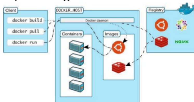
Fig. 1. Docker architecture
