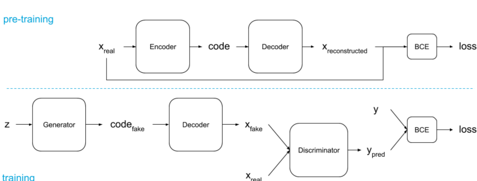
Figure 3: MedGAN [2] first pre-trains an autoencoder. During the second training phase, the decoder outputs into samples where each feature is considered as a binary variable.
