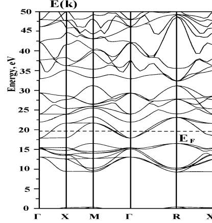
Fig. 2. Band structures for LiWO 3 .
