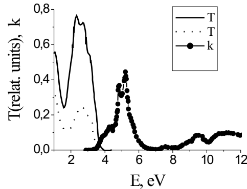
Fig. 4. Experimental transmittance spectrum of the system: \text{glass}_1/\text{ITO}/\text{WO}_3/\text{gel electrolyte}/\text{BP}/\text{ITO}/\text{glass}_2 . (Solid line – bleached, dot line – colored). Calculated parameter of absorption ( k ) of \text{LiWO}_3 .
