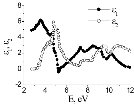
Fig. 3. Imaginary (2) and real (1) part of permittivity of \text{LiWO}_3 .
