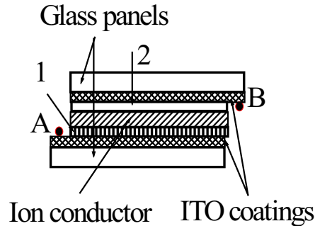
Fig. 1. Schematic representation of the assembling of the electrochromic device. Electrochromic layer (1) is WO 3 , counter electrode (2) is Prussian blue film, A and B – silver-way.
