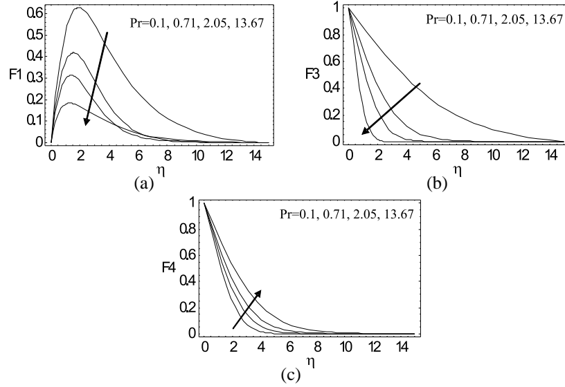
Fig. 4. The velocity (a), temperature (b) and concentration (c) profiles for Gr = 1 , Gc = 0.1 and Sc = 1 .
