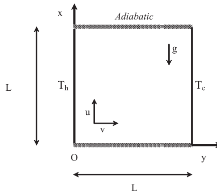
Fig. 1. Physical configuration.
