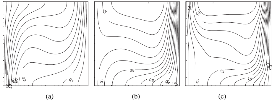
Fig. 4. Isotherms for \eta = 0 , Gr = 20000 , Pr = 0.732 and different S : (a) S = 1 ; (b) S = 10 ; (c) S = 25 .
