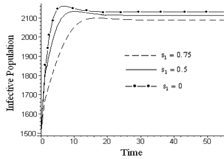
Fig. 9. Variation of infective population for different s_1 , the control parameter.
