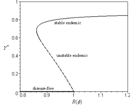
Fig. 2. Bifurcation diagram of the model system (4).
