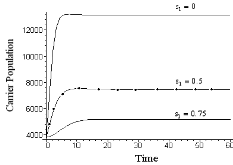
Fig. 8. Variation of carrier population for different s_1 , the control parameter.
