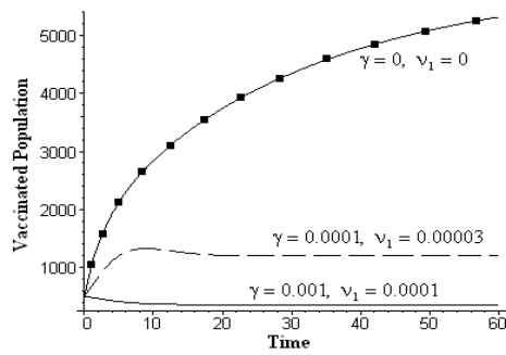
Fig. 11. Variation of vaccinated population for different values of \gamma and \nu_1 .
