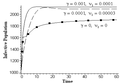
Fig. 12. Variation of infective population for different values of \gamma and \nu_1 .
