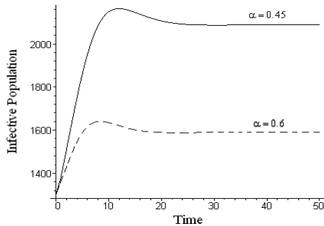
Fig. 13. Variation of infective population for different values of disease induced-death rate \alpha .
