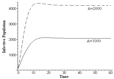
Fig. 14. Variation of infective population for different rates of immigration A .
