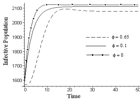
Fig. 6. Variation of infective population for different values of vaccination rate \phi .
