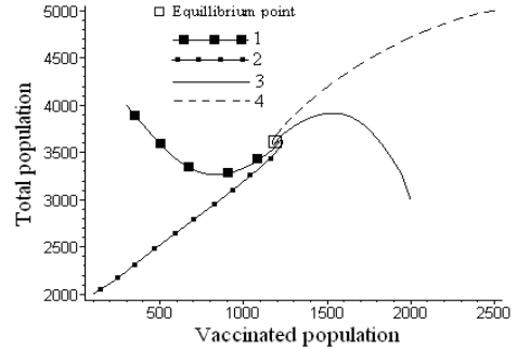
Fig. 5. Variation of total human population with vaccinated population.
