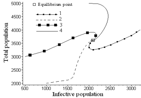
Fig. 4. Variation of total human population with infective population.
