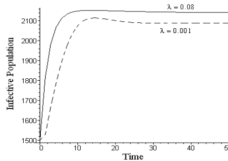
Fig. 10. Variation of infective population for different values of contact rate \lambda .
