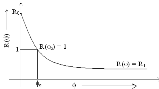
Fig. 3. Variation of vaccine induced reproduction number R(\phi) with vaccination coverage \phi .
