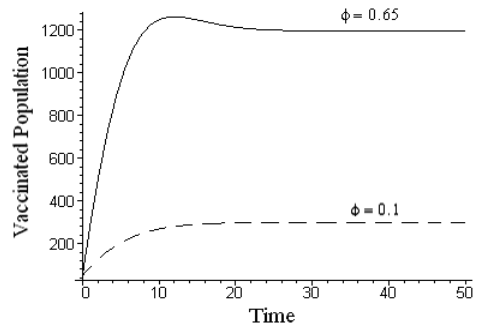
Fig. 7. Variation of vaccinated population for different values of vaccination rate \phi .
