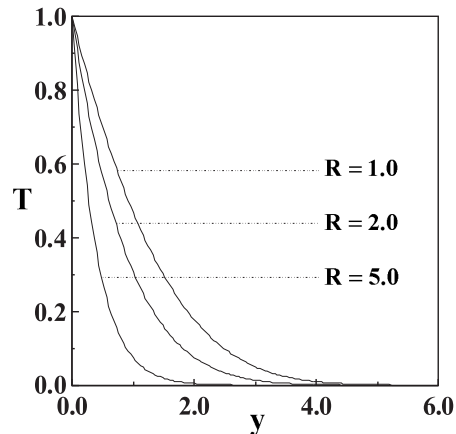
Fig. 7. Temperature profiles over a range of R with Pr = 0.5 and k = 5.0 .
