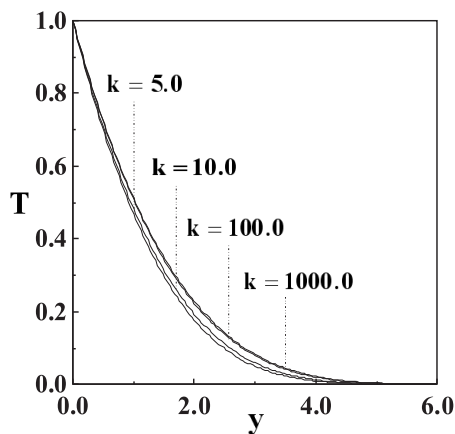
Fig. 6. Temperature profiles over a range of k with Pr = 0.5 and R = 1.0 .
