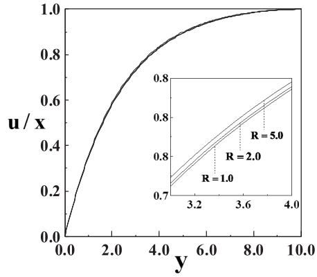
Fig. 3. Tangential velocity profiles over a range of R with k = 5.0 .
