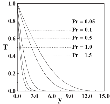
Fig. 8. Temperature profiles over a range of Pr with k = 10.0 and R = 1.0 .
