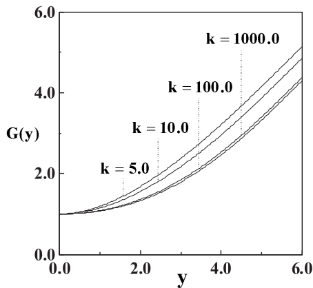
Fig. 4. Normal velocity profiles over a range of k with R = 1.0 .
