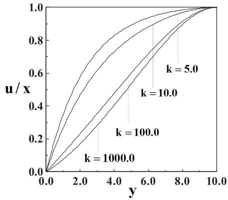
Fig. 2. Tangential velocity profiles over a range of k with R = 1.0 .
