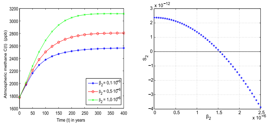
Figure 4. Variation in atmospheric concentration of methane with respect to time for different values of \beta_2 .
