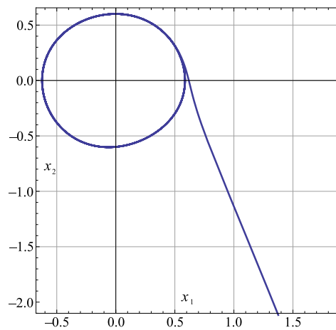
Figure 1. The VDP oscillator has one limit cycle when \mu_1 = 0.0001 , \mu_2 = -0.0001 , \mu_3 = -0.0001 , \eta = -0.1 , \delta = 0.1 with the initial values x_1(t) = -0.001 , y(t) = 0.01 for t \leq 0 .
