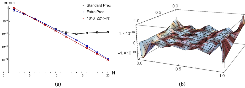
Figure 1. (a) Error in infinity norm for different values of N for equispaced nodes with standard and extra precision. (b) Three-dimensional plot of the errors is shown with N = 10 , equispaced nodes and standard precision are used (u(x_i, t_j) - u_N(x_i, t_j)) .
