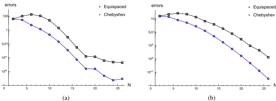
Figure 2. The errors for different values of N for equispaced (squares) and Chebyshev nodes (circles) with normal precision (a) and extra precision (b).
