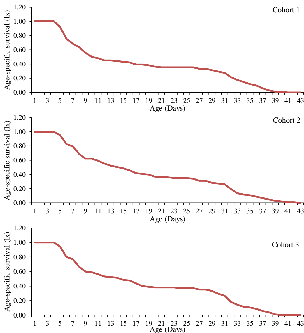
Figure 1. Survivorship curves of three cohorts of C. medinalis reared on rice plant
