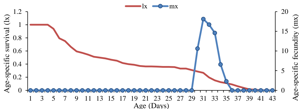
Figure 2. Daily age-specific survival ( l_x ) and fecundity ( m_x ) of female C. medinalis
