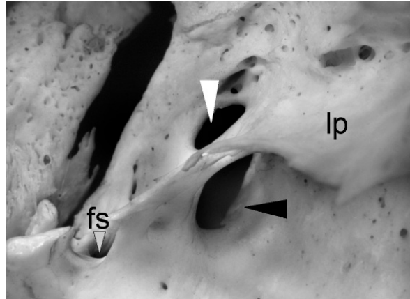
Figure 3. Magnification of the inferior view of the foramen described. The black arrow indicates the lateral compartment (oval canal; canalis ovalis ) and the white arrow indicates the medial compartment of the apparent foramen ovale; fs — foramen spinosum, lp — lateral pterygoid.
