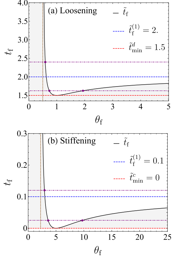
FIG. 2. Minimum connecting time as a function of the target temperature, as given by Eq. (10). Two values of the target stiffness are considered: (a) \kappa_f = 0.25 and (b) \kappa_f = 5 . The greyed area corresponds to the forbidden region t_f < \tilde{t}_f . On both panels, \tilde{t}_f is nonmonotonic and displays an absolute minimum \tilde{t}_{\min}^{d \text{ or } c} at temperatures \theta_f^d = 1 and \theta_f^c = \kappa_f . Note that \tilde{t}_{\min}^d \neq 0 whereas \tilde{t}_{\min}^c = 0 : it is impossible to engineer an instantaneous adiabatic process when loosening.
