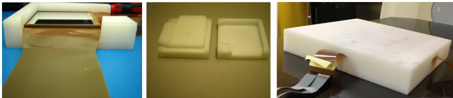
Figure 2: The final version of the dual SSSSD chip (on the left) for radiotherapy verification, placed in a polyethylene box (in the middle), which is designed to be coupled to different phantoms (on the right).
