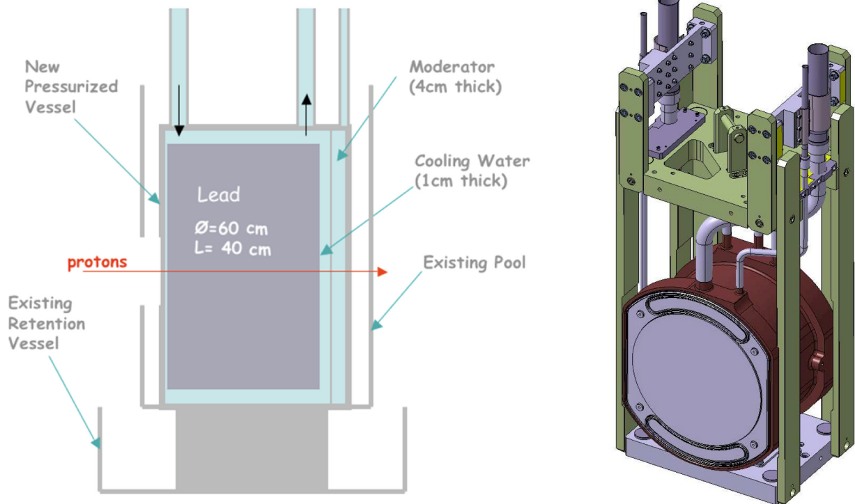
FIGURE 1. A schematic view of the upgraded lead spallation target as installed for the n_TOF facility.
