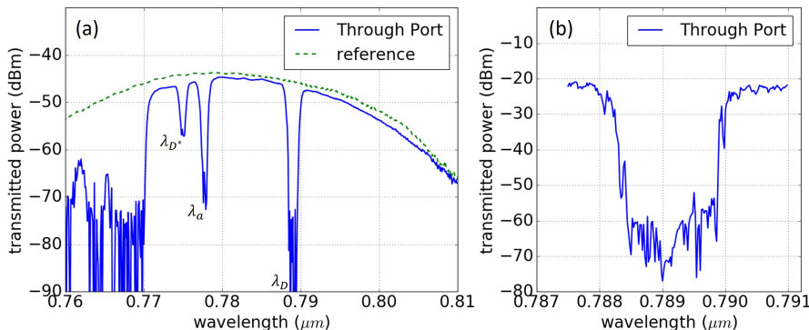
Figure 2. Measured through-port transmission spectra of a fabricated GACDC device: (a) measured with a supercontinuum source in a wide wavelength range, (b) a high resolution zoom-in measurement with a Ti:Sapphire tunable CW laser.
