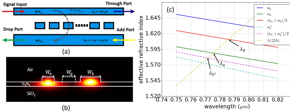
Figure 1. (a) Schematic top view of the proposed GACDC. (b) Cross-sectional with the simulated intensity distribution of the fundamental TE-like modes in the rib waveguides. (c) Dispersion curves of the modes. Phase matching wavelengths are indicated with arrows.
