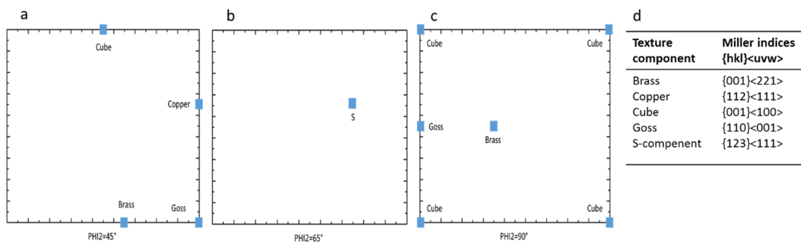
Figure 7. A key for the main texture components in FCC metals. (a) \Phi = 45^\circ ; (b) \Phi = 65^\circ ; (c) \Phi = 90^\circ and (d) a table with the Miller indices of the main texture components.
