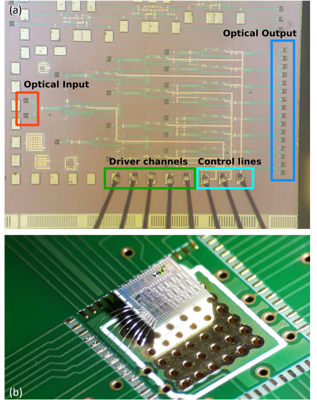
Fig. 5. (a) Microscope picture of the 3 \times 15 multicast network shown in Fig. 2(b). (b) The mounted and wirebonded chip.
