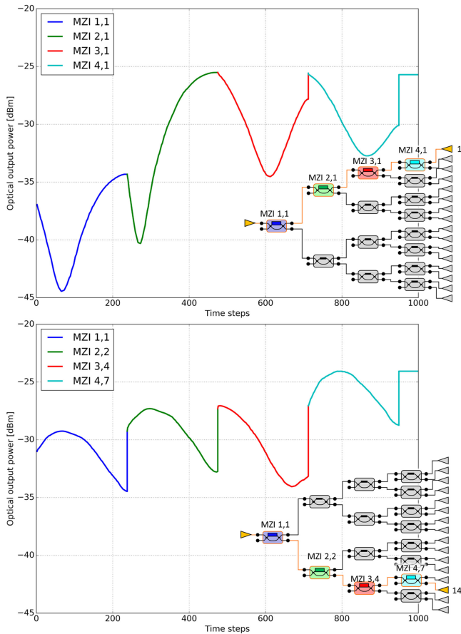
Fig. 7. Time trace of the powers in the 4 heaters as we configure the 1 \times 16 circuit to direct the input to one particular output. We perform a sweep of the D.C. along the path where the light has to go. After each sweep, the heater is set to its optimum value, and the next level in the tree is swept.
