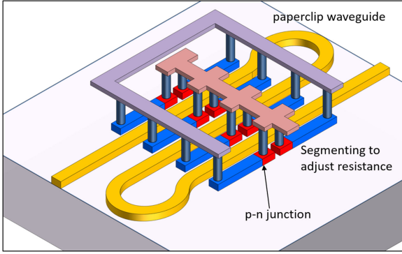
Fig. 1. Thermo-optic phase shifter using doped silicon resistors with an embedded p-n junction next to the waveguide [14]. The resistors are segmented to tune the overall resistance (and power that can be delivered for a given voltage), and the waveguide runs 3 times in between the resistors for maximum thermal efficiency.
