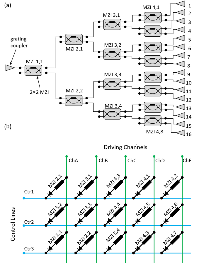
Fig. 2. (a) 1 \times 16 splitter tree circuit consisting of 15 tunable couplers, each of which is a balanced Mach-Zehnder interferometer with a thermo-optic phase shifter in one arm. (b) Electrical connectivity of the 15 thermo-optic phase shifters. They contain a diode in series and are connected to 3 control lines and 5 driver channels.
