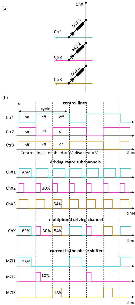
Fig. 3. Time multiplexing the signals on the driving channels. (a) A single driving channel ChX connecting three MZIs to control lines. (b) The control lines are each enabled during one third of a cycle. The subchannels ChX1 - ChX3 are modulated with a PWM duty cycle corresponding to the power that needs to be delivered to the corresponding MZIs. The subchannels are multiplexed onto the driving channel ChX synchronized with the control signals. The power is delivered to the MZIs during the corresponding parts of the cycle. Note that the control lines are at high voltage V+ when disabled, and at 0 V when enabled.
