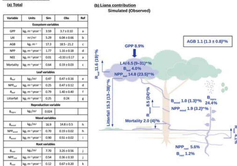
Figure 1 Total forest carbon pools and fluxes (left panel) and liana contributions (right panel). The table shows simulated (Sim) and observed (Obs) values for Paracou and the corresponding references (Ref). The sketch shows simulated liana contributions, with observed liana contributions in parentheses. B, biomass; GPP, gross primary productivity; NEE, net ecosystem exchange (negative values mean carbon uptake); NPP, net primary productivity; R, respiration. References for observations: a Paracou, French Guiana (Aguilos et al., 2018); b Paracou, French Guiana (TLS data, this study); c Paracou, French Guiana (Rutishauser, Wagner, Haurault, Nicolini, & Blanc, 2010); d Paracou, French Guiana (Longo et al., 2019); e Paracou, French Guiana (Domenach et al., 2004); f Paracou, French Guiana (Stahl, 2010); g Paracou, French Guiana (De Weirdt et al., 2012); h Paracou, French Guiana (Baker et al., 2004); i Paracou, French Guiana (Stahl, Burban, Goret, &
