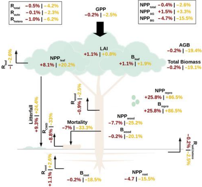
Figure 5 Relative changes in carbon pools and fluxes for Paracou, French Guiana (brown), and Gigante, Panama (yellow), upon inclusion of the liana plant functional type in the simulations. B, biomass; GPP, gross primary productivity; NPP, net primary productivity; R, respiration
