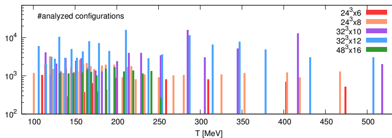
Figure 1. Number of the analyzed lattice configurations.
