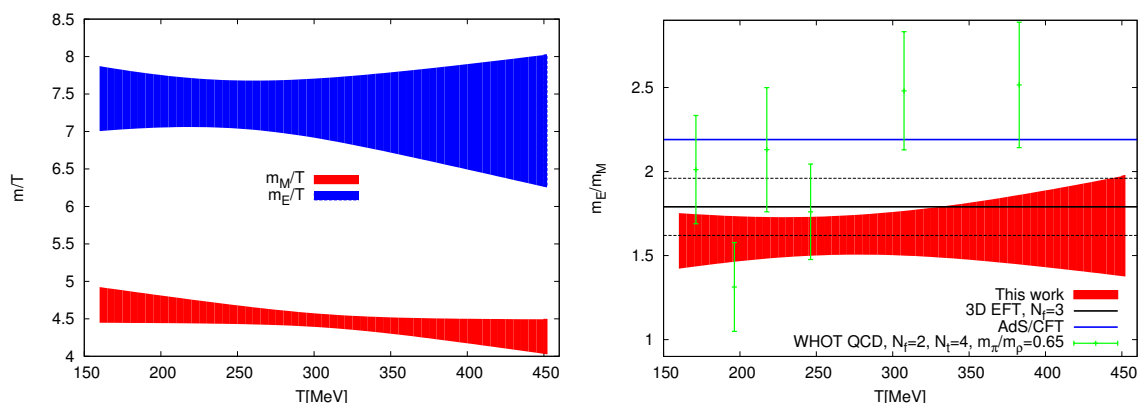
Figure 9. The continuum extrapolations of the screening masses and the ratio of the screening masses. For the ratio m_E/m_M we also included different estimates from the literature: lattice results from ref. [32], dimensionally reduced 3D effective field theory results at T = 2T_c from ref. [43], and results from \mathcal{N} = 4 SYM plasma with AdS/CFT from ref. [44].
