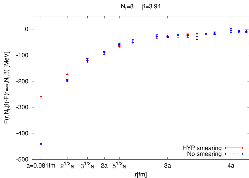
Figure 2. The smeared and unsmeared free energies at a given \beta and N_t , after the first step of the renormalization procedure.
