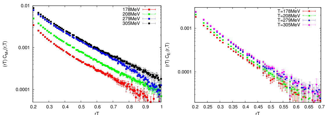
Figure 7. Illustrating that the screening masses are approximately proportional to the temperature. Since the x axis of this plot is rT , if one assumes a Yukawa form of the correlator, than the slopes of these curves are just m_M/T and m_E/T respectively. The fact that the graphs are approximately parallel straight lines suggests that these ansatzes are approximately correct, and that the masses are approximately proportional to the temperature.
