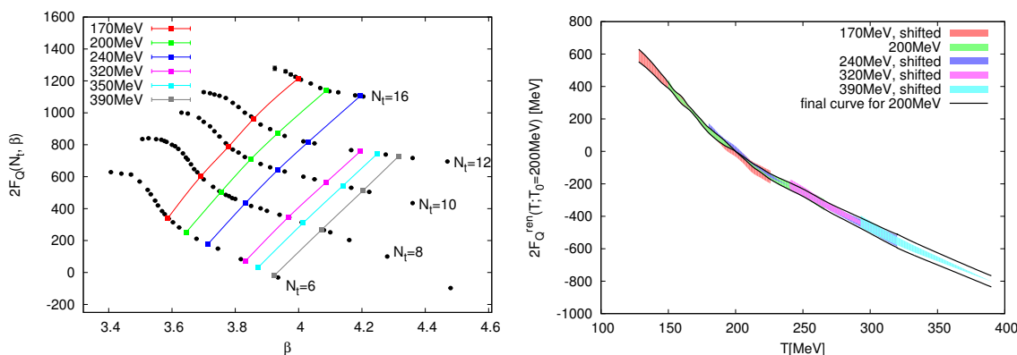
Figure 3. Left: determining F_Q(\beta, T_0) for different values of T_0 with interpolation. The bare 2F_Q values for different values of N_t are the black symbols. The colored symbols correspond to different fixed T_0 values for each N_t . The colored lines are interpolations between these points in \beta . Right: 2F_Q^{\text{ren}}(T; T_0) values in the continuum, calculated for different values of T_0 . For the final curve, all of the curves have been shifted to the position of the T_0 = 200 MeV curve. The errors of each piece decrease as we approach the corresponding T_0 . For the final curve, we used linear error propagation, assuming independent errors. We also mention that calculating the continuum limit of 2F_Q^{\text{ren}}(T; T_0) without HYP smearing leads to results consistent with the one presented here.
