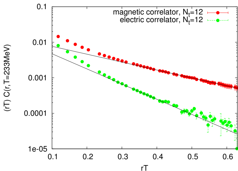
Figure 6. Illustrating m_E > m_M with the lattice data at N_t = 12 and T = 233 MeV ( 32^3 lattices with HYP smearing). It can be clearly seen that the electric correlator drops faster. To lead the eye, we included on the plot the Yukawa fits to the tails of the correlators.
