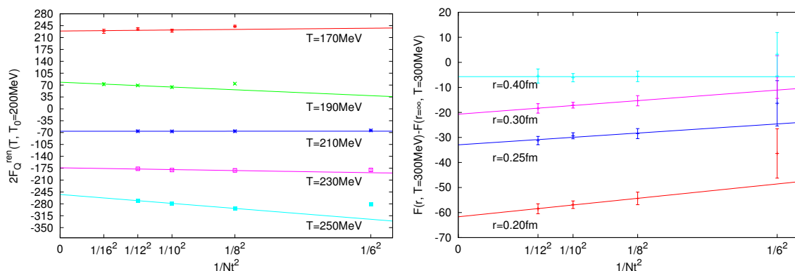
Figure 5. Cut-off effects in the free energy. On the left, we see an illustration of the continuum extrapolation of the renormalized single heavy quark free energy, with T_0 = 200 MeV, at different temperature values. As can be seen from a closer inspection of this figure, the cut-off error in this quantity, at these lattice spacings is approximately 5–10%. On the right, we can see a continuum extrapolation of \tilde{F}_{\bar{Q}Q}(r, \beta, T) = F_{\bar{Q}Q}(r, \beta, T) - F_{\bar{Q}Q}(r \rightarrow \infty, \beta, T) at T = 300 MeV, for different values of r . Cut-off effects have a similar magnitude here as well.
