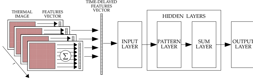
Fig. 1. An overall schema of the feature extraction and classification process. Starting from thermal images singular feature vectors are extracted. Groups of 4 consecutive feature vectors are joined and used as input for a radial basis function neural network.
