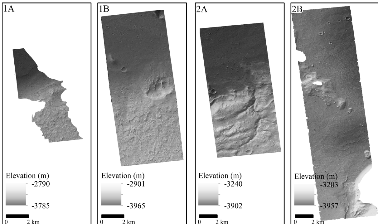
Fig. 5. Results of the DTM production process. Location of particular DTMs corresponds to common extents of each stereo pair as marked in Fig. 1
