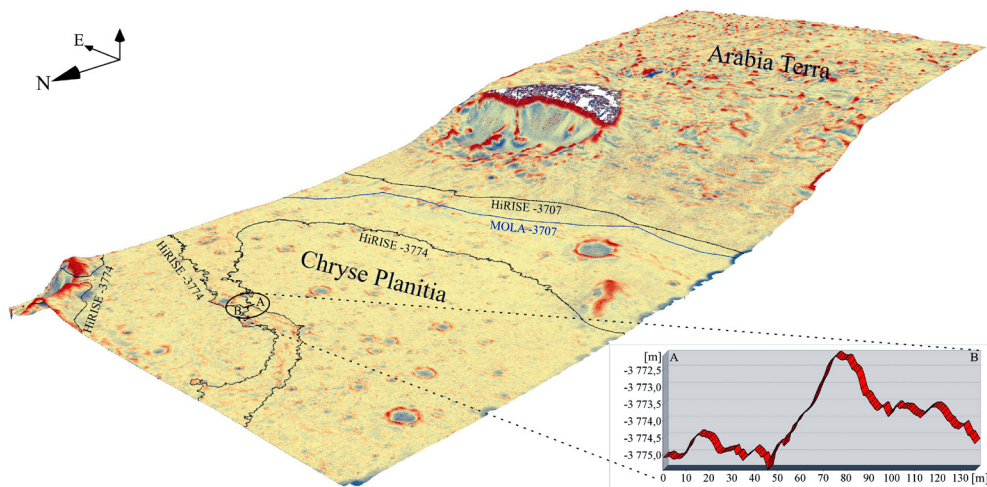
Fig. 6. Perspective view of area 1B composed of draped TPI on HiRISE DTM. Vertical exaggeration \times 2 . Red areas are convex, blue areas concave with regard to their surroundings. Dark grey contours represent elevation from HiRISE DTM, the blue one represents elevation from MOLA DTM
