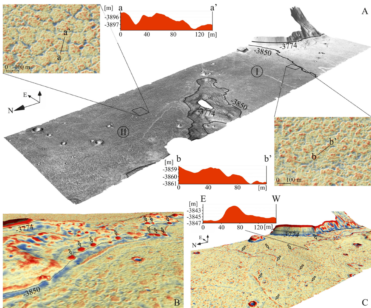
Fig. 9. Perspective views of 2B. Vertical exaggeration x3
