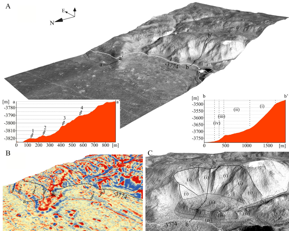
Fig. 7. Perspective views of area 2A. Vertical exaggeration \times 3 .
