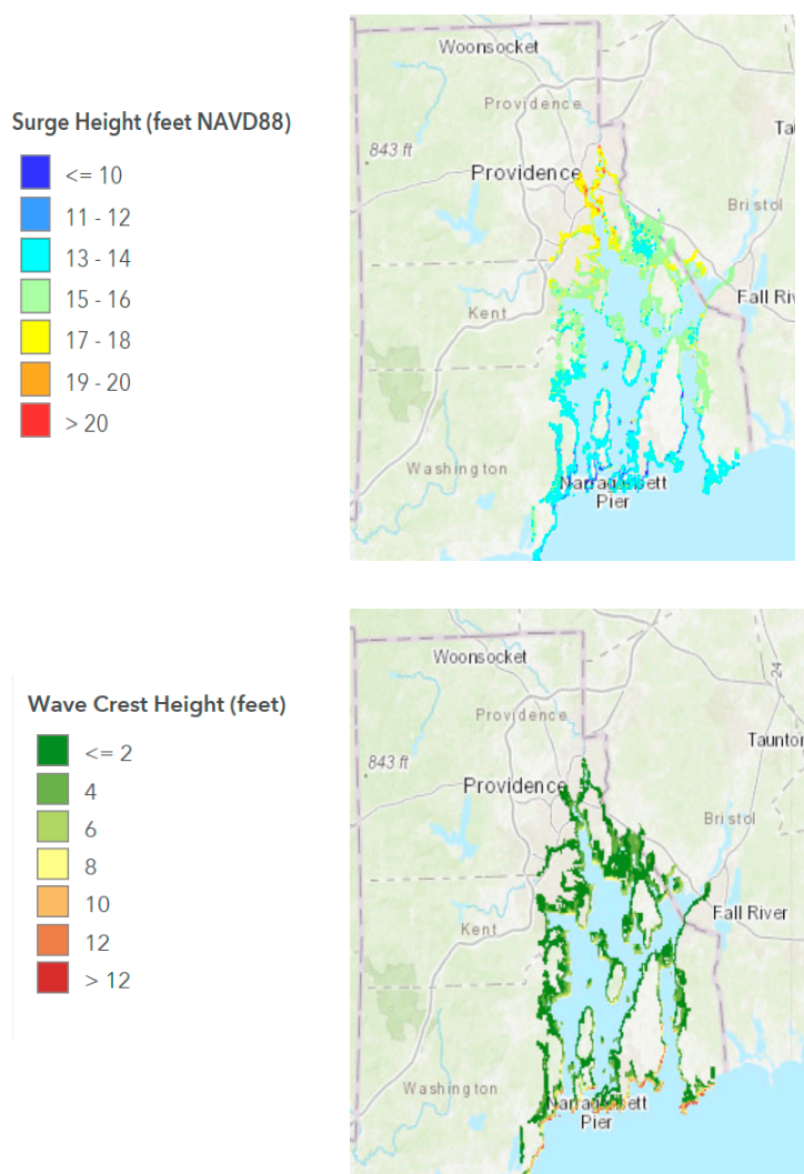
Figure 12. Surge inundation levels (relative to NAVD88) (upper panel) and the wave crest height (lower panel) for Narragansett Bay for 100-yr, no-SLR case.
