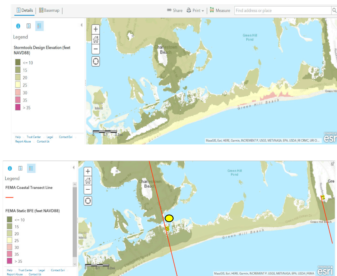
Figure 9. Comparison of SDE (upper panel) vs. FEMA FIRM (lower panel) BFE maps for the 100-yr, no-SLR case. Yellow dot indicates the location of the comparative analysis shown in Table 2.
