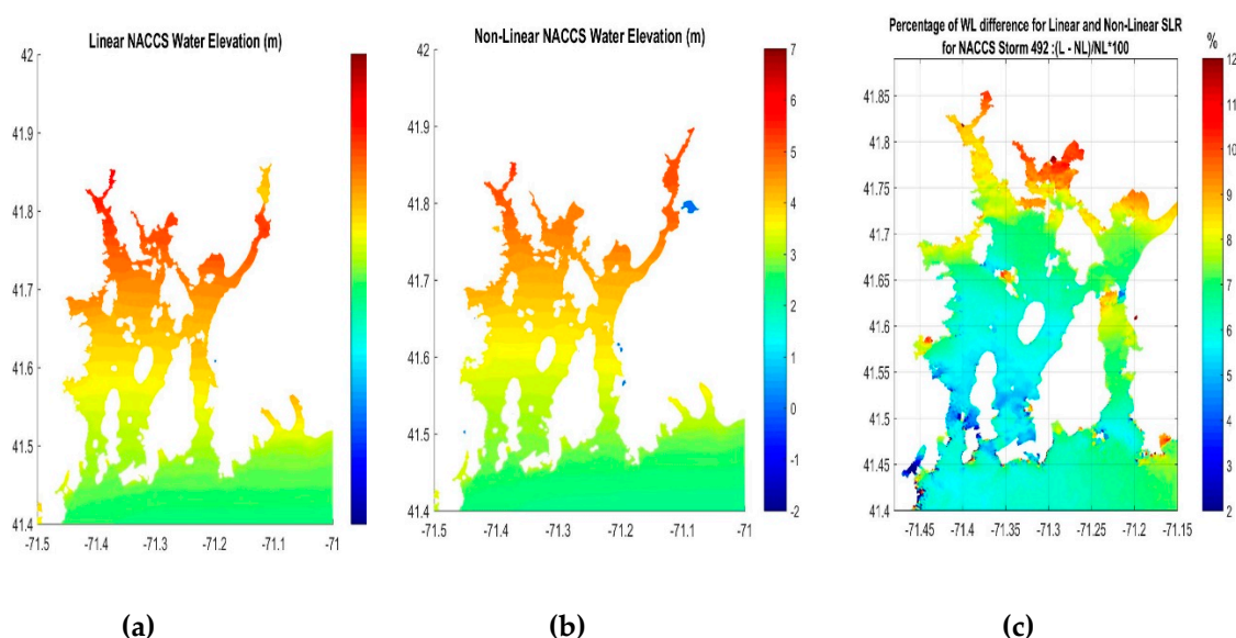
Figure 4. Peak water level for NACCS storm #492 for Narragansett Bay for (a) linear superposition method, (b) full nonlinear simulation results, and (c) percent (%) difference between the two for 6.6-ft (2-m) SLR.
