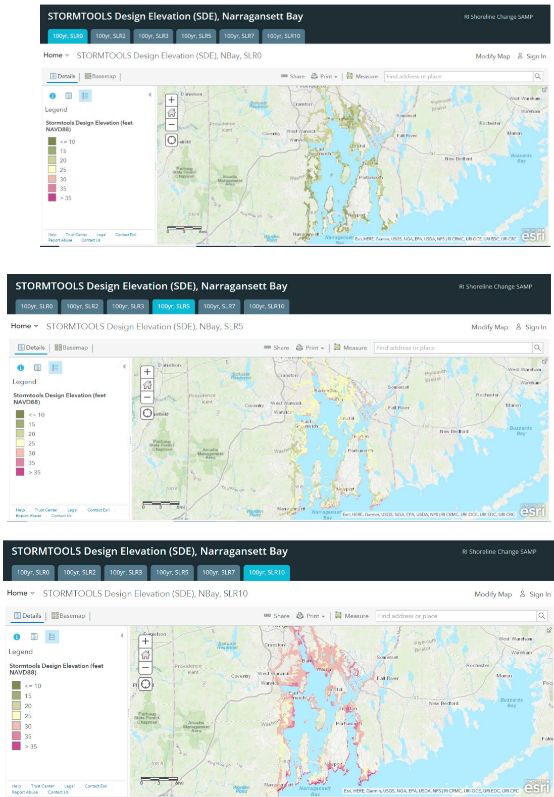
Figure 11. Impact of SLR on Narragansett Bay SDE maps, cases shown are 0, 5 ft (1.52 m), and 10 ft (3.05 m) SLR (upper, middle, and lower panel, respectively).
