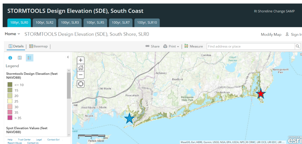
Figure 5. User interface for the STORMTOOLS Design Elevation (SDE) Maps, southern RI coast line (South Coast), no SLR. The case selected was the 100-yr event with no SLR. Blue star, Napatree Point, Westerly, and red star, Point Judith, South Kingstown. The units on the tab are in ft of SLR. ( https://crc-
