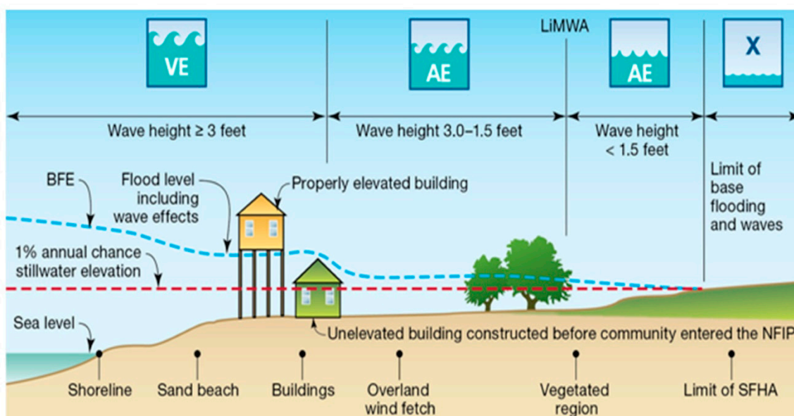
Figure 1. FEMA flood zone map definitions. Dashed red line is the 1% inundation level and the dashed blue line is the base flood elevation (BFE). These can be referenced to as either grade elevation or NAVD88 benchmarks. Zone definitions are provided at the top of the figure (VE, AE, LIMWA, and X). ( http://www.r3coastal.com/home/coastal-hazard-analysis-mapping/coastal-flood-hazard-mapping , accessed on 11 February 2020). (Definition of the flood zones are provided at https://www.fema.gov/flood-zones , accessed on 16 April 2020.)
