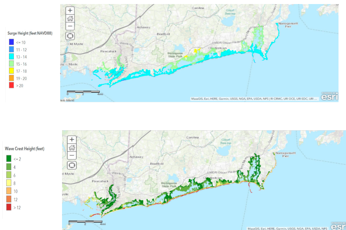
Figure 7. Surge inundation levels (relative to NAVD88) (upper panel) and the wave crest height (lower panel) for southern coast of RI for 100-yr, no-SLR case.
