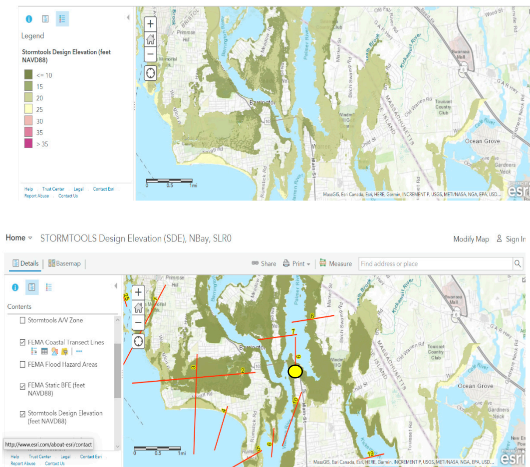
Figure 14. Comparison of SDE (upper panel) vs. FEMA (lower panel) BFE maps for the 100-yr, no-SLR case. The FEMA transect lines are shown in the FIRM maps.
