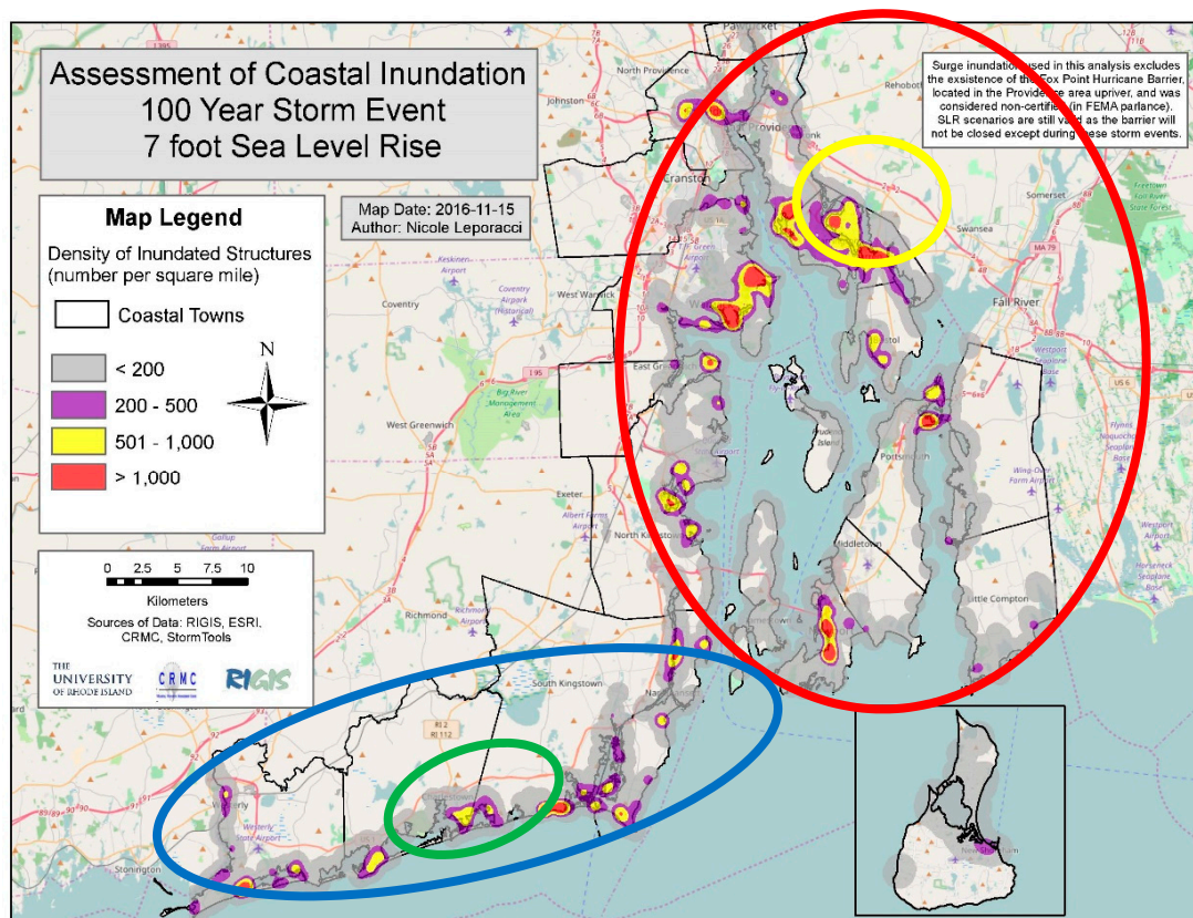
Figure 2. Density of structures inundated with 100-yr storm surge plus 7 ft (2.1 m) sea level rise (SLR) for Narragansett Bay, RI, and the southern coast of RI based on STORMTOOLS. The red and blue ovals show the Narragansett Bay and southern RI shoreline study areas, respectively. The green oval shows the location of Charlestown, RI, and the yellow oval the towns of Barrington, Warren and Bristol, RI. study areas ( http://www.beachsamp.org/wpcontent/uploads/2016/11/Map_SLR7_100YR_Edited_11_15.jpg , accessed, 26 October 2017).
