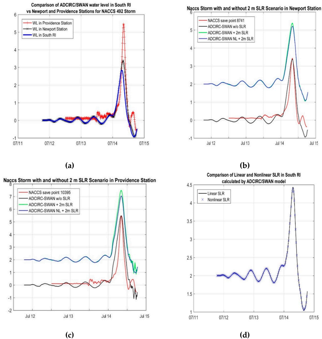
Figure 3. (a) Water level vs. time for NACCS storm #492 at Providence, Newport, and Charlestown, RI; (b) ADCIRC-SWAN-predicted water level vs. time for NACCS storm #492 at Newport without sea level rise (SLR), with 6.6 ft (2 m) of SLR simply added on, and with 2-m SLR added to the initial bathymetry and simulations run with the full model, (c) same as in (b) but at the Providence station; and (d) results of linear (superposition) and nonlinear simulation at Charlestown.
