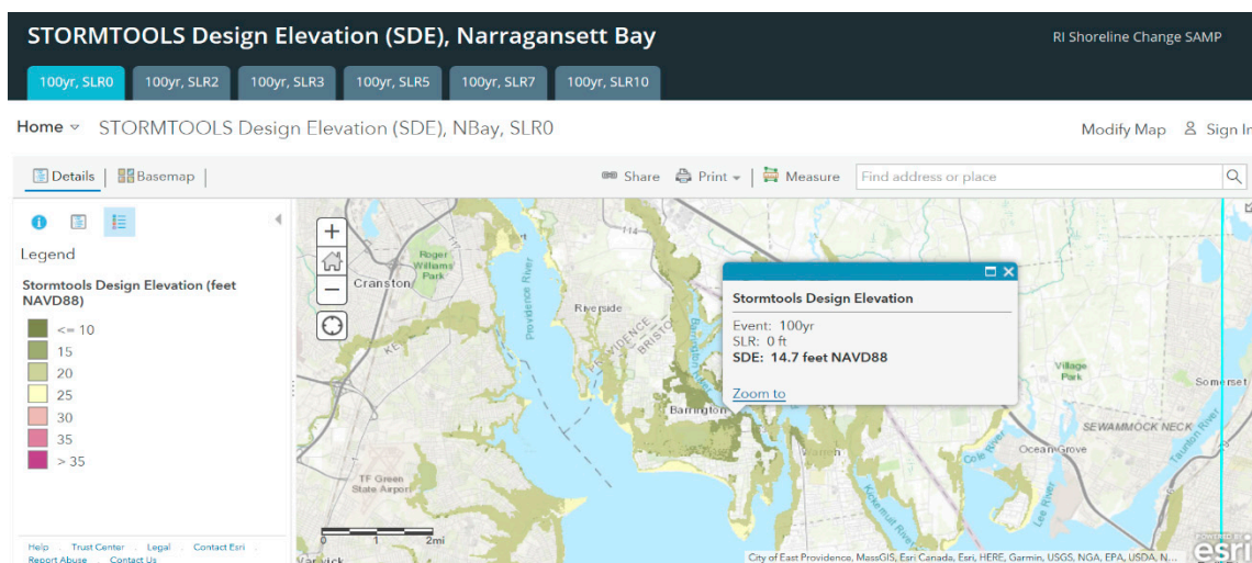
Figure 13. Flooding in the vicinity of Barrington, Warren, and Bristol, RI, for 100-yr, no-SLR case. The point interrogation tool was used to determine the BFE at the location selected.
