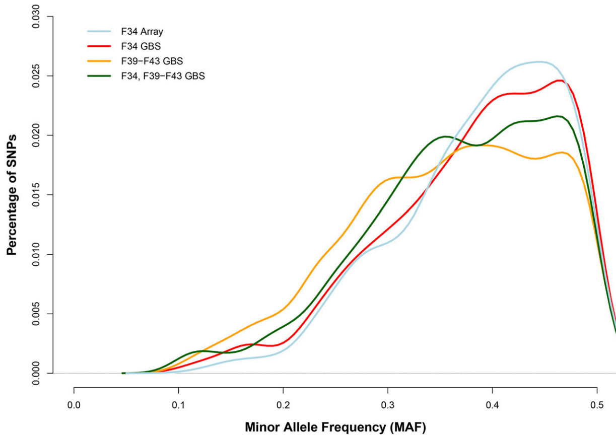
Figure 1 Minor allele frequency (MAF) distributions for F_{34} array, F_{34} GBS, F_{39-F43} GBS, and F_{34} and F_{39-F43} GBS SNP sets. The average MAF of those 4,593 array SNPs was 0.388; the average MAF of the 60,392 GBS-derived SNPs in 428 F_{34} AIL mice was 0.382; the average MAF of the 59,790 GBS-derived SNPs in 600 F_{39-43} AIL mice was 0.358; the average MAF of the 58,461 GBS-derived SNPs that existed in both F_{34} and F_{39-43} AIL mice was 0.370 (Table S2). MAF distributions are highly comparable between AIL generations.
