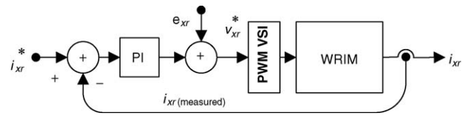
Fig. 1. Current control loop ( x=d, q ).
