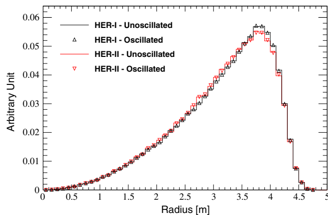
FIG. 9. Comparison of the radial distributions from unoscillated and oscillated neutrinos in the HER-I and HER-II ranges. Oscillated and unoscillated spectra are almost indistinguishable, confirming the negligible dependence of the radial distribution on the energy spectrum. The MSW-LMA parameters used for simulating oscillating neutrinos are \Delta m^2 = 7.50 \times 10^{-5} \text{ eV}^2 , \sin^2(\theta_{12}) = 0.306 , and \sin^2(\theta_{13}) = 0.02166 [29].
