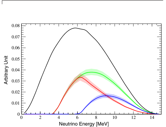
FIG. 13. Response functions from Eq. (A2) for i = e, x corresponding to the HER (green), HER-I (red), and HER-II (blue) energy ranges, respectively. The black line is the ^8\text{B} neutrino spectrum, for reference.
