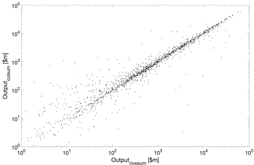
Figure 1 Rocket plot of outputs calculated via row sum and column sum in 2015.
