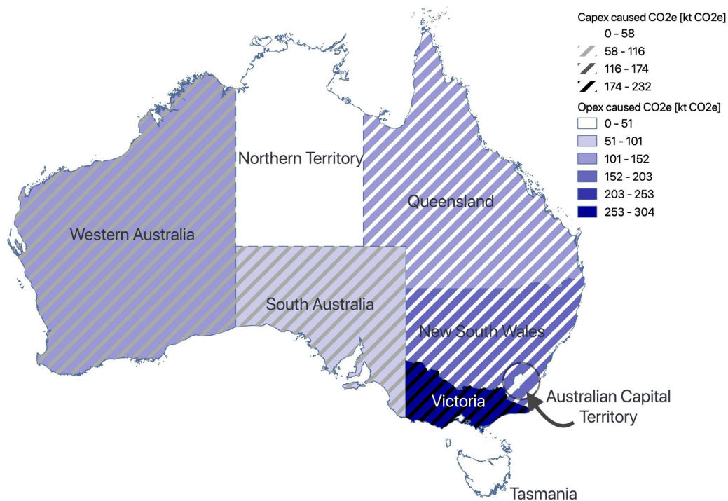
Figure 3 CO 2 e emissions by states and territories caused by capex and opex in 2012.
