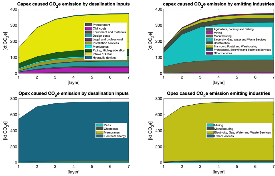
Figure 5 Production layer decomposition for desalination inputs and emitting industries in 2012.
