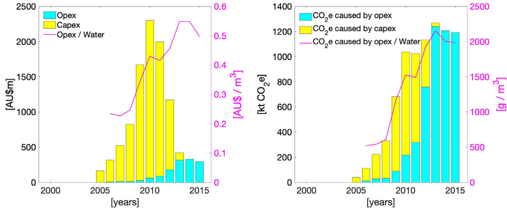
Figure 2 Overview of costs and CO 2 e emissions.
