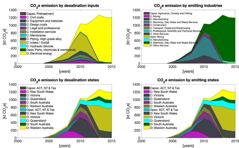
Figure 4 CO 2 e emission by desalination inputs and emitting industries.
