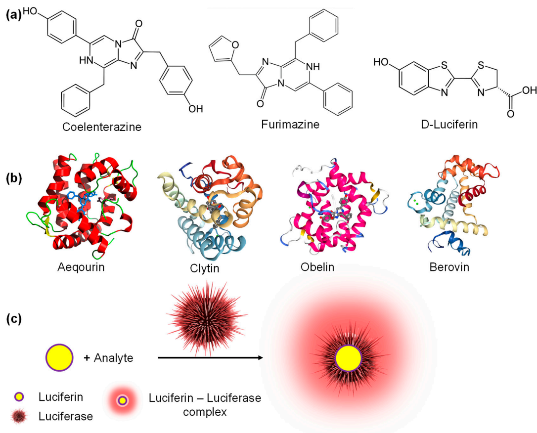
Figure 9. (a) Small molecules as luciferins; (b) Photoproteins; (c) Bioluminescence with a luciferin-luciferase assembly.
