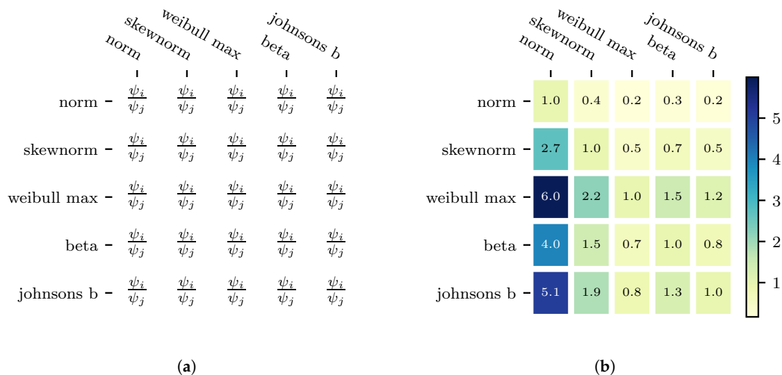
Figure 6. Visualization of the Probability distribution model selection step in the uncertainty analyzer framework for the impact factor. The PDFM-ratio of the probability distribution models is shown in the left plot (a), with the corresponding results of the case study in the right plot (b). The greater the value in the right plot, the more accurate is the probability distribution model of the row (j) compared to the probability distribution model of the column (i). The probability distribution model is selected corresponding the row that has the highest values when comparing all columns.
