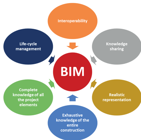
Fig. 1 BIM principles
