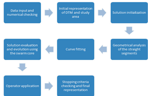
Fig. 5 Optimization algorithm
