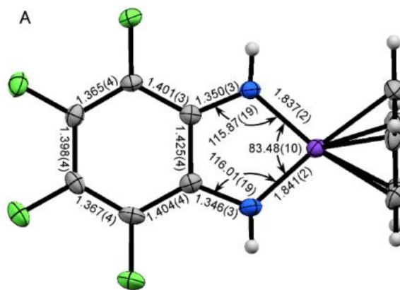
Figure 1. Molecular structure of one (A) of four crystallographically independent molecules with bond distances (Å) and angles (deg); thermal ellipsoids are at the 50% probability level.
