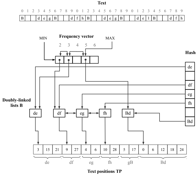
Figure 2: The low-frequency queue is composed by three components: frequency vector, hash, and doubly-linked lists. In this example, the text is obtained from abcdegabdcdfhabcdegabcde labcdfh after the substitutions (in order) A \rightarrow ab and B \rightarrow Ac . Pairs de , df , eg , fh , and Bd have been inserted in the queue. We do not show F - and L -fields in B 's elements to improve readability.
